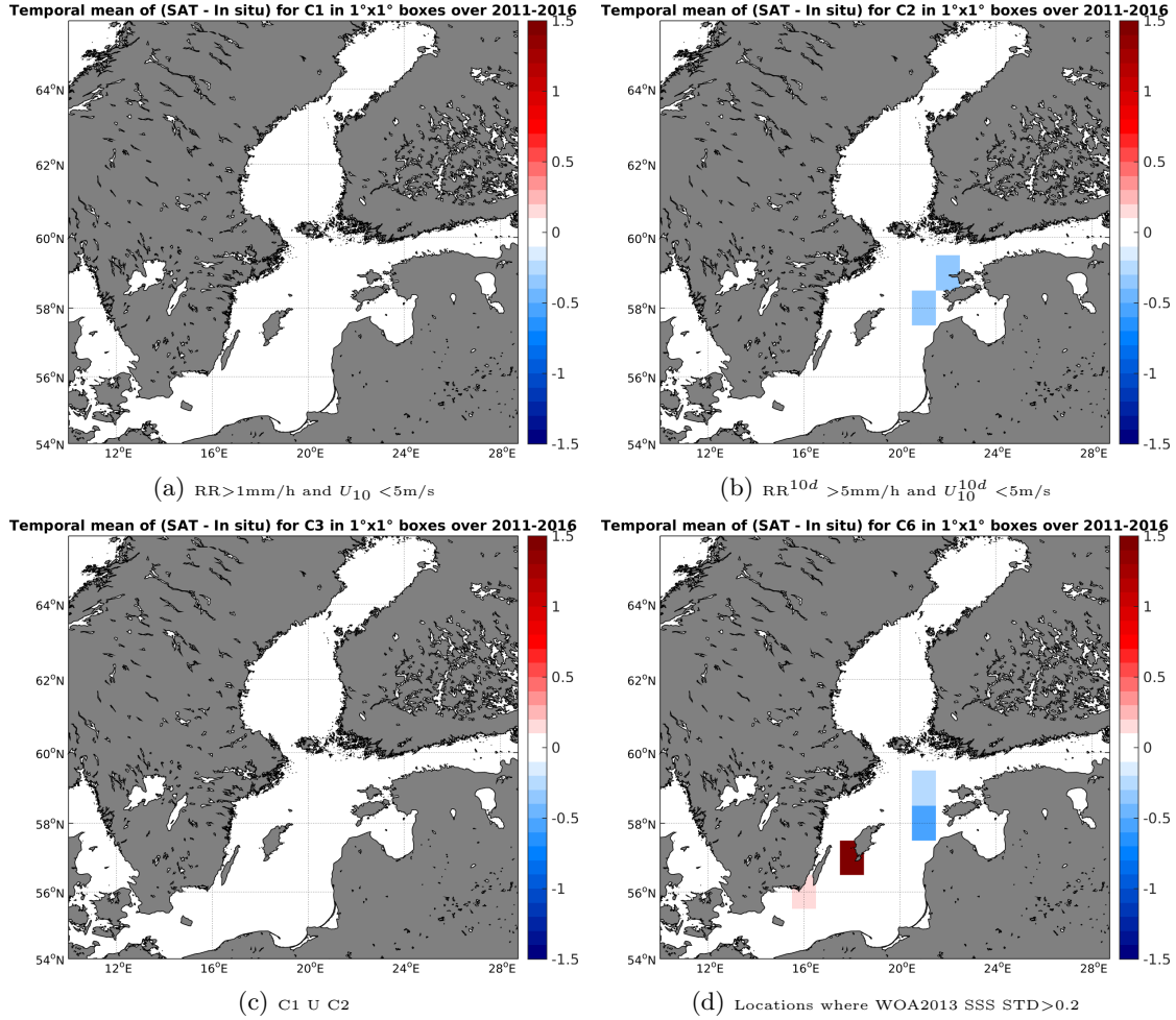
Figure 12: Temporal mean gridded over spatial boxes of size 1°x1° of \Delta SSS (SMOS-L3-CATDS-CECOS-LOCEAN-V2-9DAYS-25KM - TSG-LEGOS-DM) for 4 different subdatasets corresponding to: RR > 1\text{mm/h} and U_{10} < 5\text{m/s} (a), RR^{10d} > 5\text{mm/h} and U_{10}^{10d} < 5\text{m/s} (b), C1 U C2 (c), Locations where WOA2013 SSS STD > 0.2 (d).
