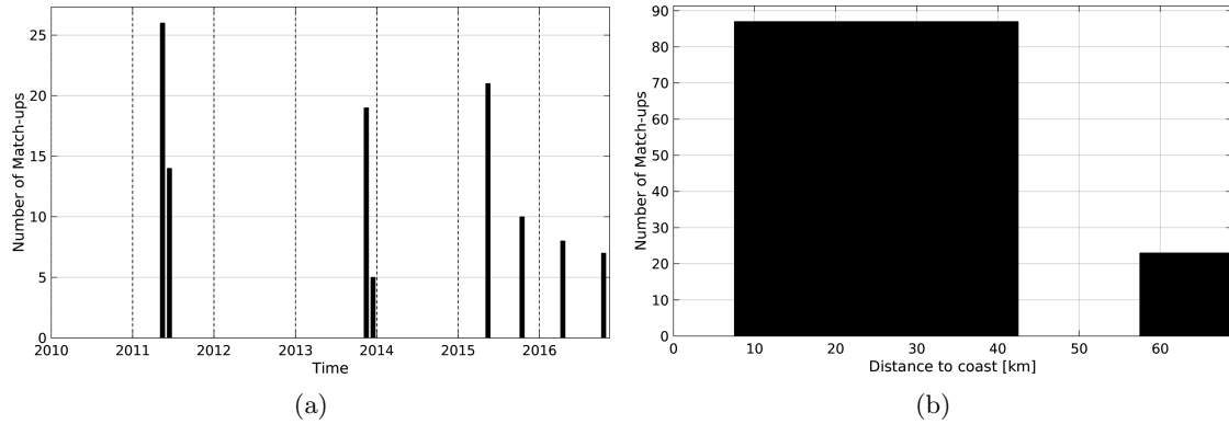
Figure 1: Number of match-ups between TSG-LEGOS-DM and SMOS-L3-CATDS-CECOS-LOCEAN-V2-9DAYS-25KM SSS as a function of time (a) and as function of the distance to coast (b) over the Baltic Sea Pi-MEP region and for the full satellite product period.
