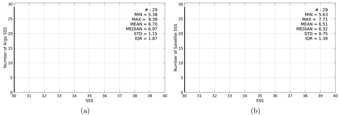
Figure 2: Histograms of SSS from Argo (a) and SMOS-L3-CATDS-CECOS-LOCEAN-V2-9DAYS-25KM (b) considering all match-up pairs per bins of 0.1 over the Baltic Sea Pi-MEP region and for the full satellite product period.
