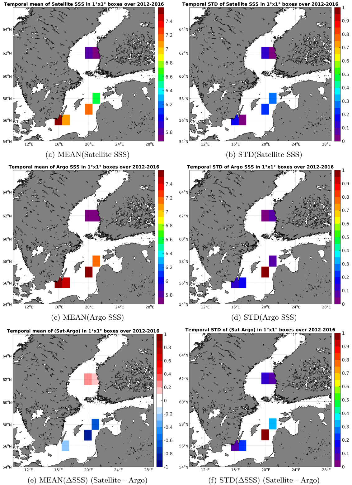
Figure 6: Temporal mean (left) and STD (right) of SSS from SMOS-L3-CATDS-CECOS-LOCEAN-V2-9DAYS-25KM (top), Argo (middle), and of \Delta SSS (Satellite - Argo). Only match-up pairs are used to generate these maps.
