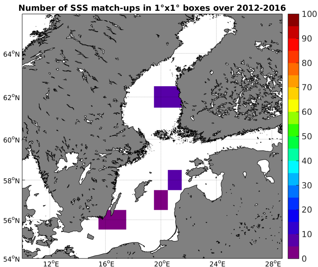
Figure 4: Number of SSS match-ups between Argo SSS and the SMOS-L3-CATDS-CECOS-LOCEAN-V2-9DAYS-25KM SSS product for the Baltic Sea Pi-MEP region over 1°x1° boxes and for the full satellite product period.
