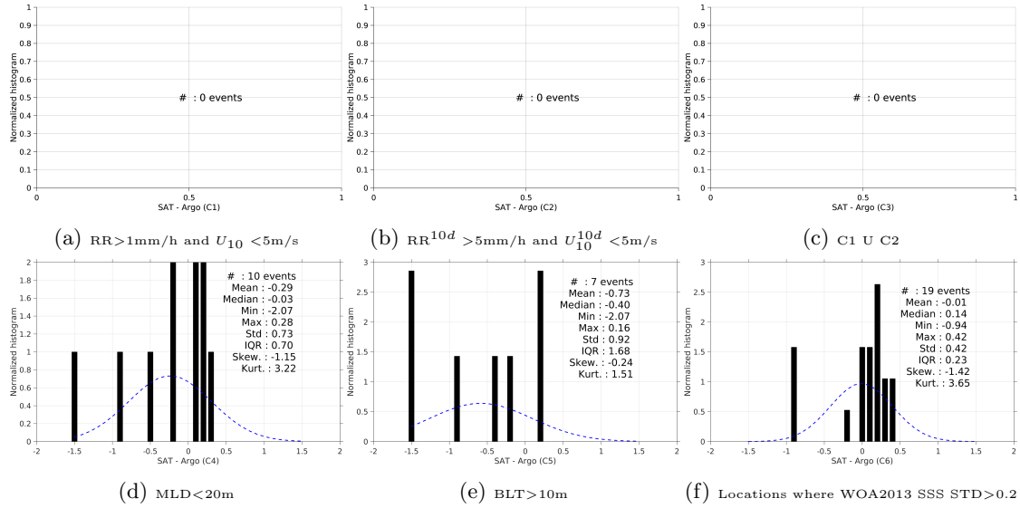
Figure 13: Normalized histogram of \Delta\text{SSS} (SMOS-L3-CATDS-CECOS-LOCEAN-V2-9DAYS-25KM - Argo) for 6 different subdatasets corresponding to: RR > 1\text{mm/h} and U_{10} < 5\text{m/s} (a), RR^{10d} > 5\text{mm/h} and U_{10}^{10d} < 5\text{m/s} (b), C1 U C2 (c), MLD < 20\text{m} (d), BLT > 10\text{m} (e), Locations where WOA2013 SSS STD > 0.2 (f).
