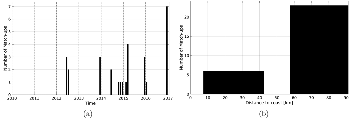
Figure 1: Number of match-ups between Argo and SMOS-L3-CATDS-CECOS-LOCEAN-V2-9DAYS-25KM SSS as a function of time (a) and as function of the distance to coast (b) over the Baltic Sea Pi-MEP region and for the full satellite product period.
