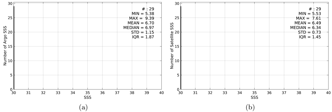
Figure 2: Histograms of SSS from Argo (a) and SMOS-L3-CATDS-CECOS-LOCEAN-V2-18DAYS-25KM (b) considering all match-up pairs per bins of 0.1 over the Baltic Sea Pi-MEP region and for the full satellite product period.
