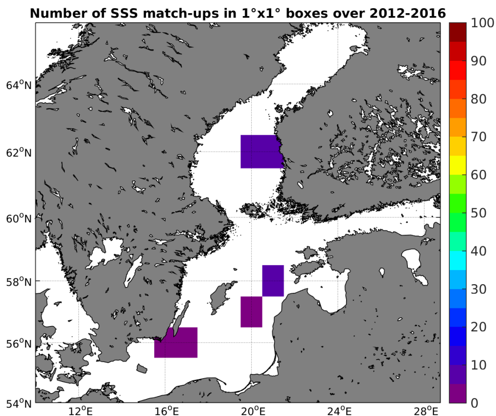
Figure 4: Number of SSS match-ups between Argo SSS and the SMOS-L3-CATDS-CECOS-LOCEAN-V2-18DAYS-25KM SSS product for the Baltic Sea Pi-MEP region over 1°x1° boxes and for the full satellite product period.
