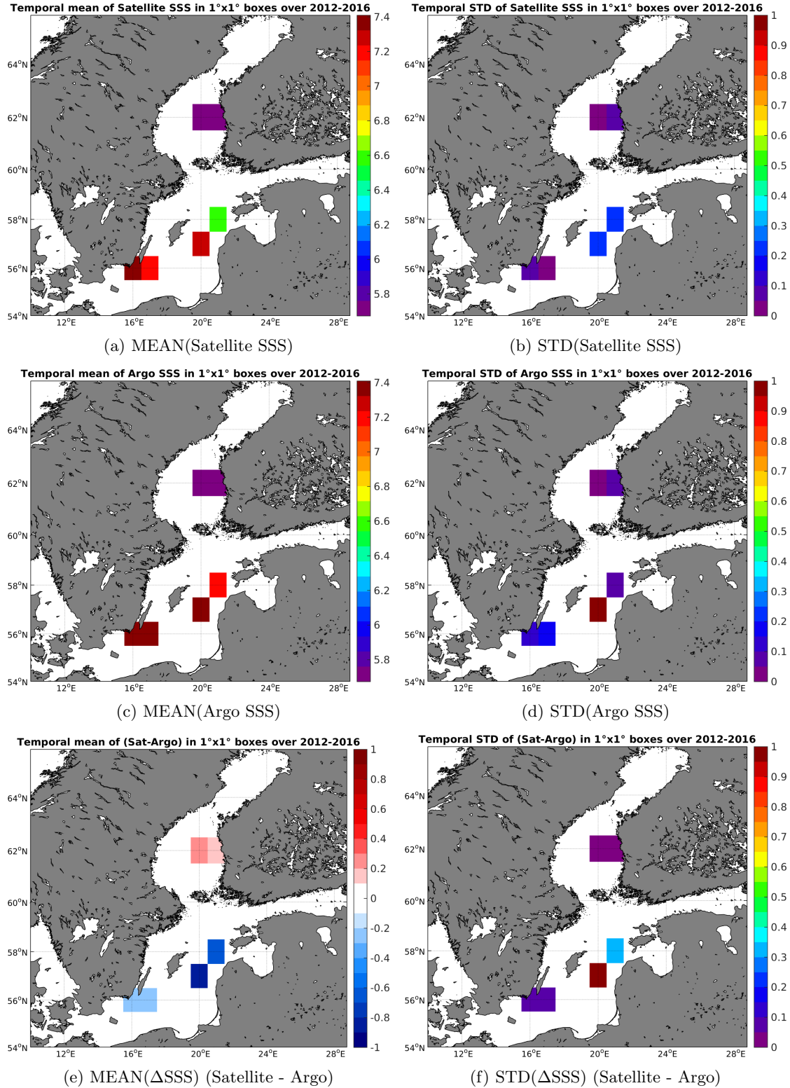
Figure 6: Temporal mean (left) and STD (right) of SSS from SMOS-L3-CATDS-CECOS-LOCEAN-V2-18DAYS-25KM (top), Argo (middle), and of \Delta SSS (Satellite - Argo). Only match-up pairs are used to generate these maps.
