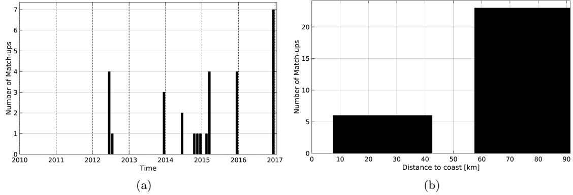
Figure 1: Number of match-ups between Argo and SMOS-L3-CATDS-CECOS-LOCEAN-V2-18DAYS-25KM SSS as a function of time (a) and as function of the distance to coast (b) over the Baltic Sea Pi-MEP region and for the full satellite product period.
