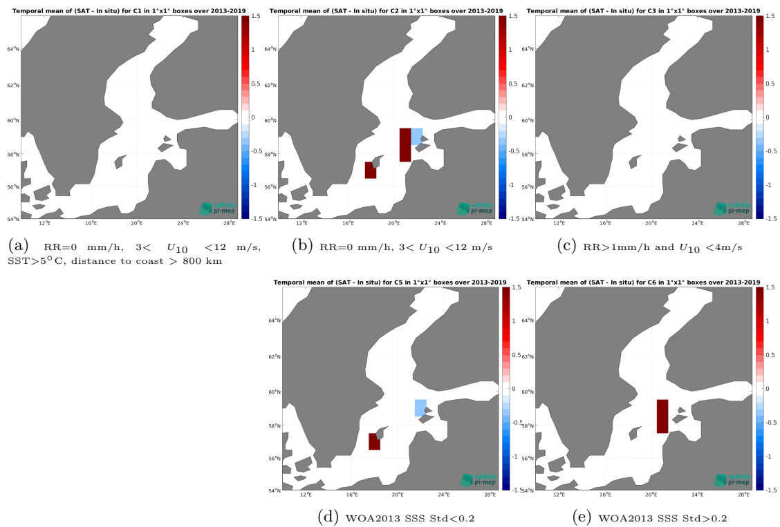
Figure 14: Temporal mean gridded over spatial boxes of size 1^\circ \times 1^\circ of \Delta SSS (SMOS SSS L3 v335 - Monthly - 25 km (CATDS-CPDC) - TSG (LEGOS-DM)) for 5 different subdatasets corresponding to:RR=0 mm/h, 3 < U_{10} < 12 m/s, SST >5^\circ\text{C} , distance to coast > 800 km (a), RR=0 mm/h, 3 < U_{10} < 12 m/s (b), RR >1 mm/h and U_{10} < 4 m/s (c), WOA2013 SSS Std <0.2 (d), WOA2013 SSS Std >0.2 (e).
