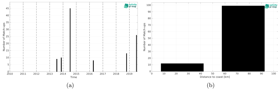
Figure 2: Number of match-ups between TSG (LEGOS-DM) and SMOS SSS L3 v335 - Monthly - 25 km (CATDS-CPDC) SSS as a function of time (a) and as function of the distance to coast (b) over the Baltic Sea Pi-MEP region and for the full satellite product period.
