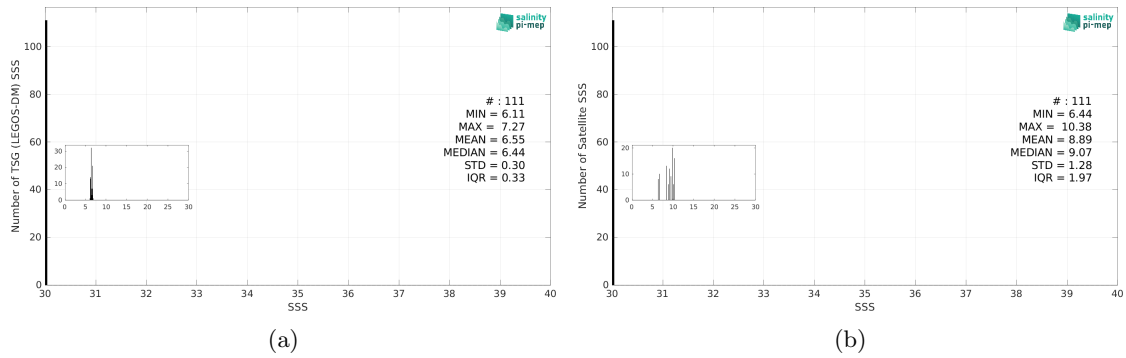
Figure 3: Histograms of SSS from TSG (LEGOS-DM) (a) and SMOS SSS L3 v335 - Monthly - 25 km (CATDS-CPDC) (b) considering all match-up pairs per bins of 0.1 over the Baltic Sea Pi-MEP region and for the full satellite product period.
