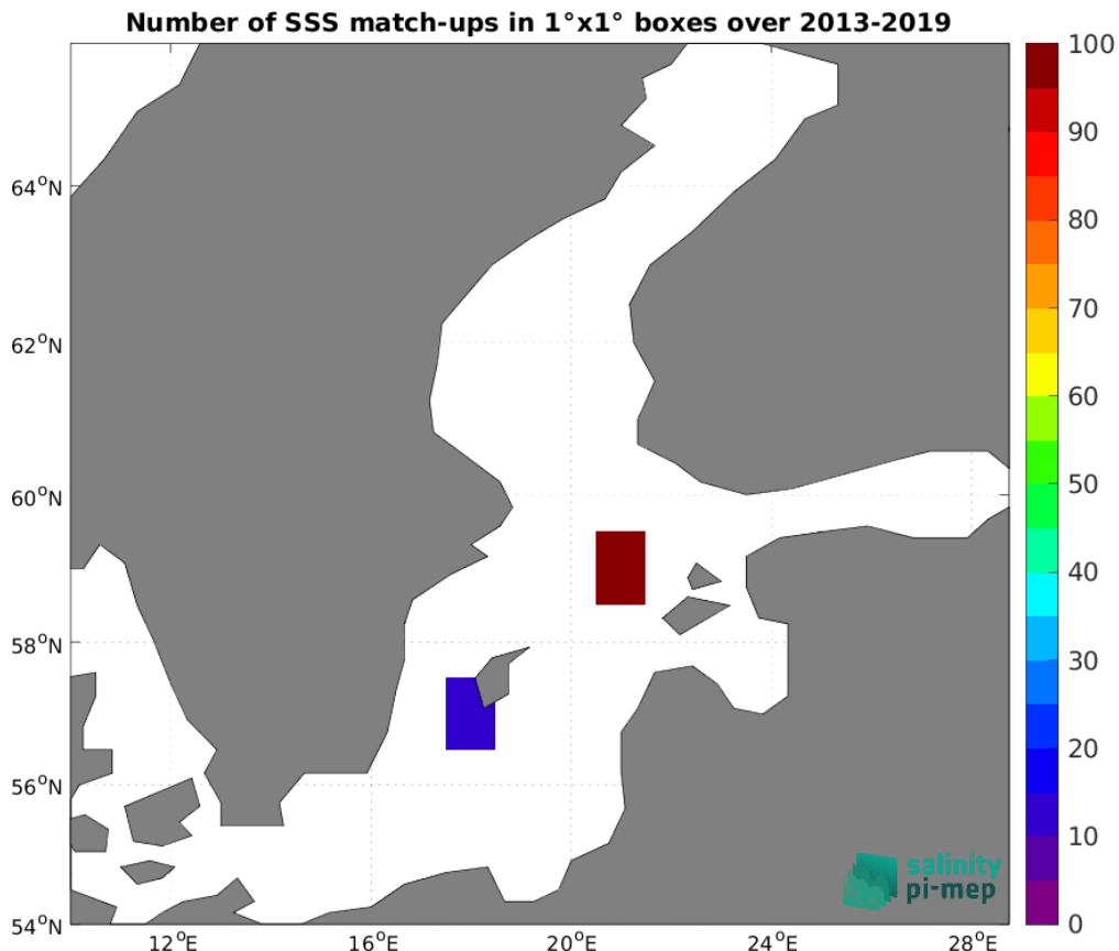
Figure 5: Number of SSS match-ups between TSG (LEGOS-DM) SSS and the SMOS SSS L3 v335 - Monthly - 25 km (CATDS-CPDC) SSS product for the Baltic Sea Pi-MEP region over 1°x1° boxes and for the full satellite product period.
