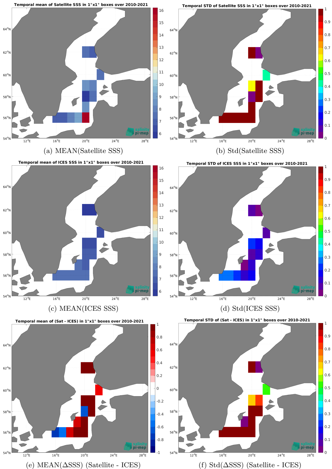
Figure 7: Temporal mean (left) and Std (right) of SSS from SMOS SSS L3 v335 - Monthly - 25 km (CATDS-CPDC) (top), ICES (middle), and of \Delta SSS (Satellite - ICES). Only match-up pairs are used to generate these maps.
