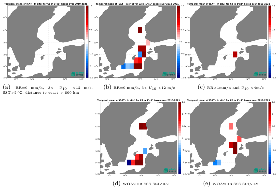
Figure 14: Temporal mean gridded over spatial boxes of size 1^\circ \times 1^\circ of \Delta SSS (SMOS SSS L3 v335 - Monthly - 25 km (CATDS-CPDC) - ICES) for 5 different subdatasets corresponding to:RR=0 mm/h, 3 < U_{10} < 12 m/s, SST >5^\circ\text{C} , distance to coast > 800 km (a), RR=0 mm/h, 3 < U_{10} < 12 m/s (b), RR >1 mm/h and U_{10} < 4 m/s (c), WOA2013 SSS Std <0.2 (d), WOA2013 SSS Std >0.2 (e).
