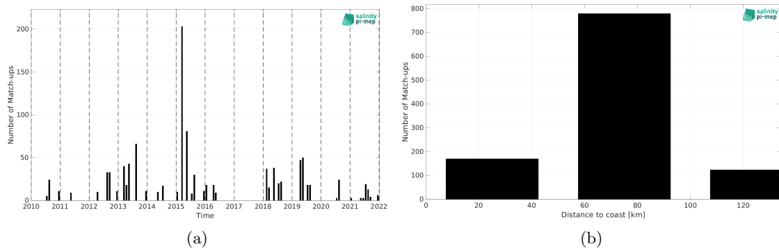
Figure 2: Number of match-ups between ICES and SMOS SSS L3 v335 - Monthly - 25 km (CATDS-CPDC) SSS as a function of time (a) and as function of the distance to coast (b) over the Baltic Sea Pi-MEP region and for the full satellite product period.
