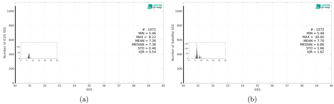
Figure 3: Histograms of SSS from ICES (a) and SMOS SSS L3 v335 - Monthly - 25 km (CATDS-CPDC) (b) considering all match-up pairs per bins of 0.1 over the Baltic Sea Pi-MEP region and for the full satellite product period.
