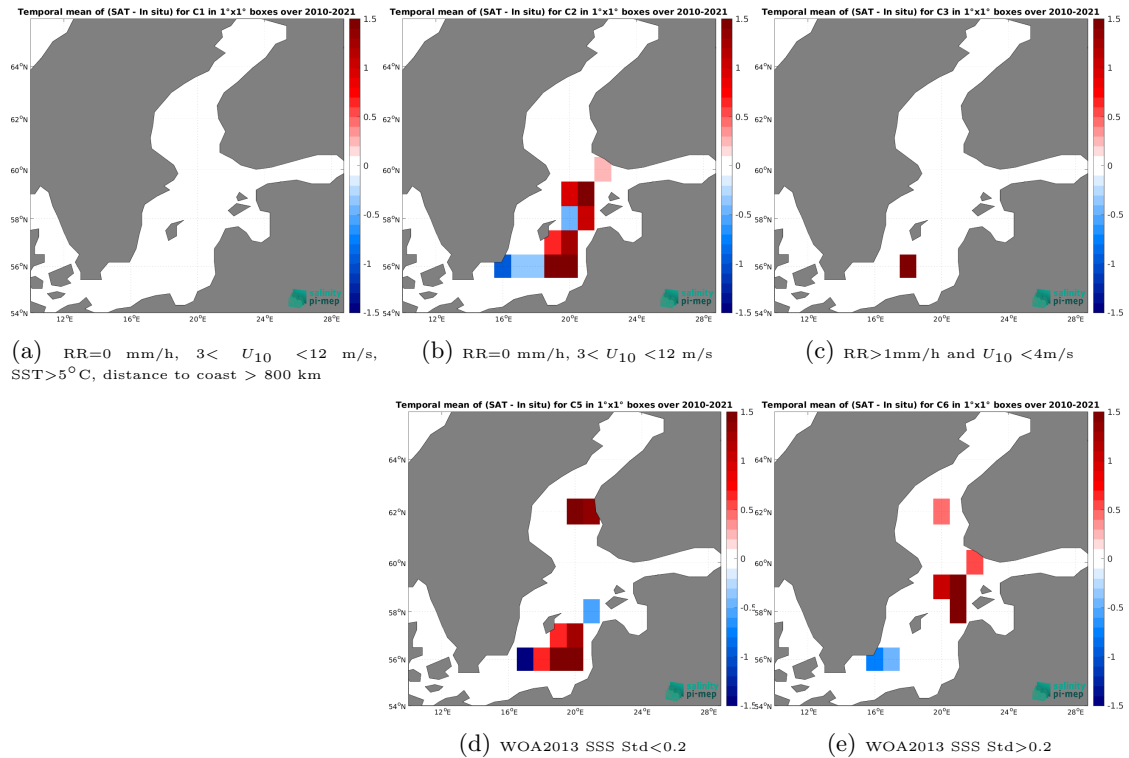
Figure 12: Temporal mean gridded over spatial boxes of size 1^{\circ}\times 1^{\circ} of \Delta\text{SSS} (SMOS SSS L3 v335 - Monthly - 25 km (CATDS-CPDC) - ICES) for 5 different subdatasets corresponding to:RR=0 mm/h, 3 < U_{10} < 12 m/s, SST > 5^{\circ}\text{C} , distance to coast > 800 km (a), RR=0 mm/h, 3 < U_{10} < 12 m/s (b), RR > 1 mm/h and U_{10} < 4 m/s (c), WOA2013 SSS Std < 0.2 (d), WOA2013 SSS Std > 0.2 (e).
