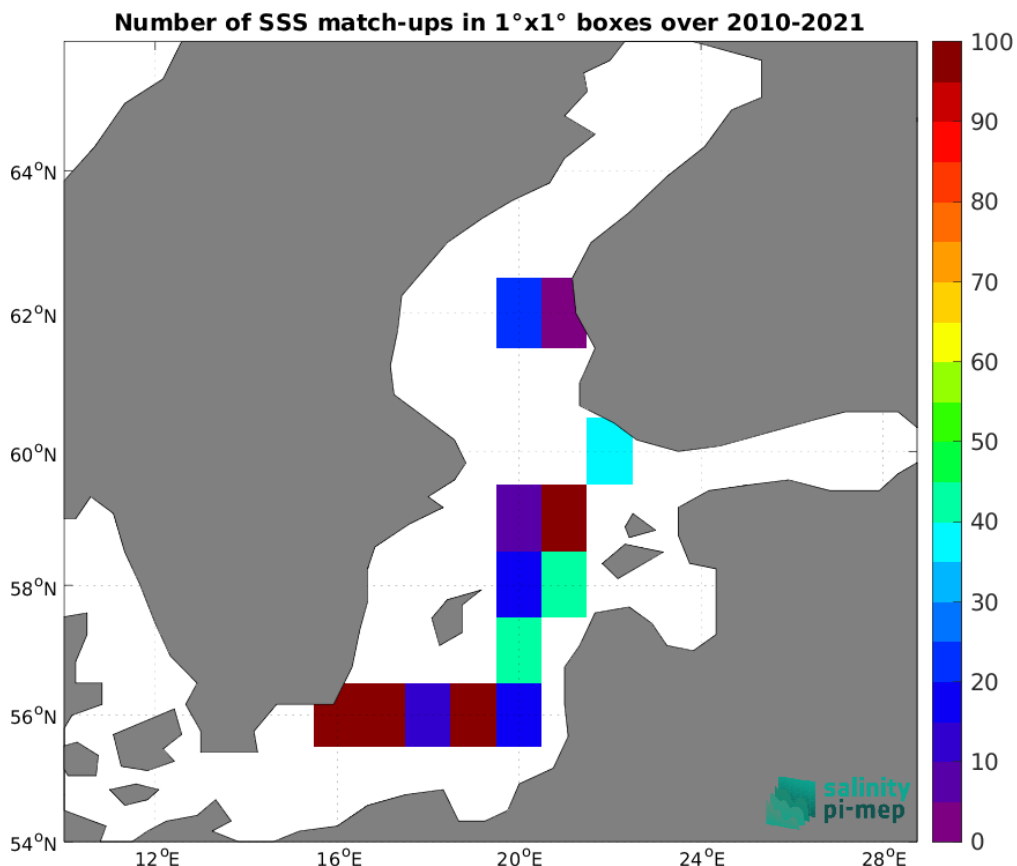
Figure 4: Number of SSS match-ups between ICES SSS and the SMOS SSS L3 v335 - Monthly - 25 km (CATDS-CPDC) SSS product for the Baltic Sea Pi-MEP region over 1^{\circ} \times 1^{\circ} boxes and for the full satellite product period.
