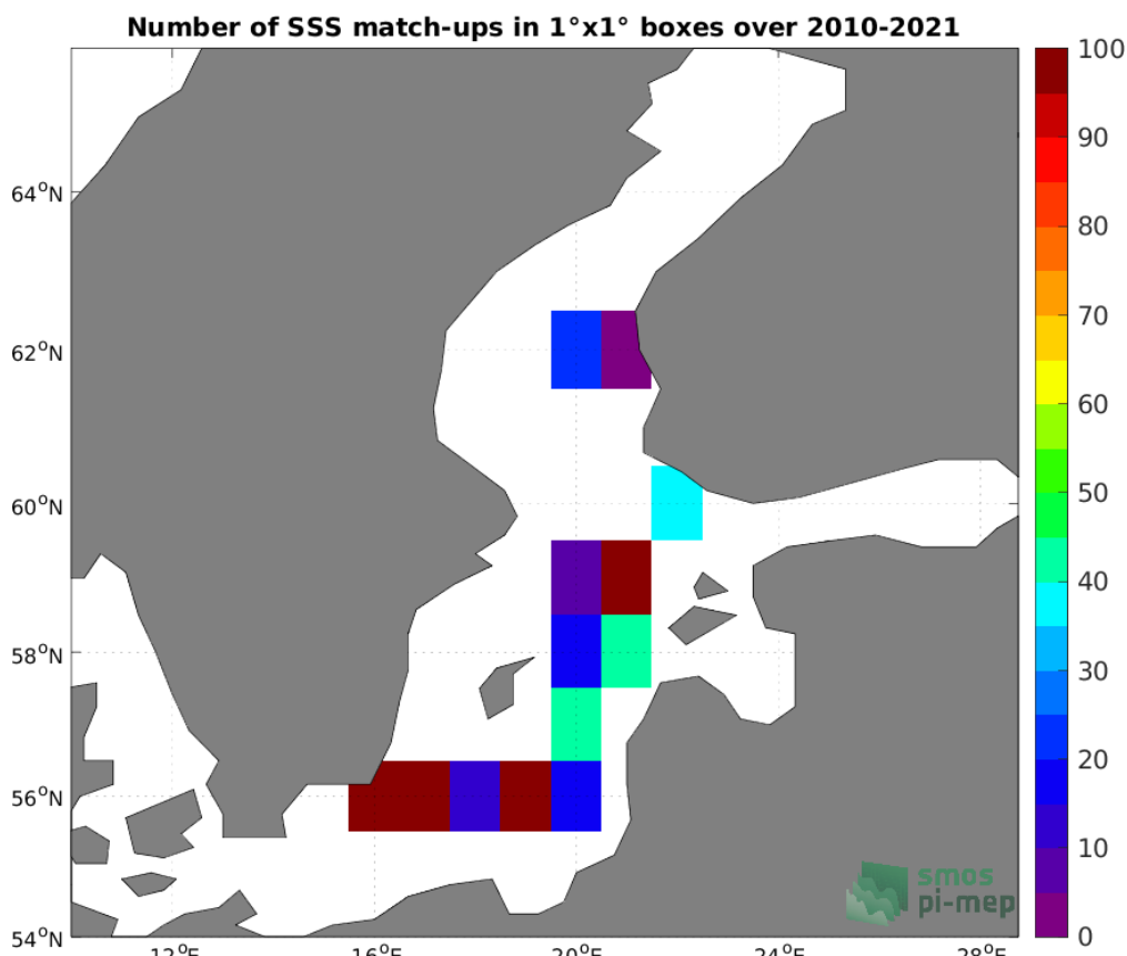
Figure 4: Number of SSS match-ups between ICES SSS and the SMOS SSS L3 v335 - Monthly - 25 km (CATDS-CPDC) SSS product for the Baltic Sea Pi-MEP region over 1°x1° boxes and for the full satellite product period.
