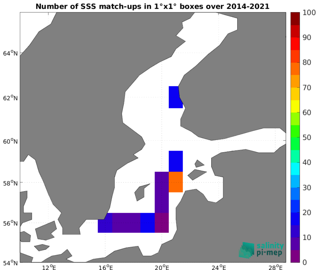
Figure 4: Number of SSS match-ups between Argo SSS and the SMOS SSS L3 v335 - Monthly - 25 km (CATDS-CPDC) SSS product for the Baltic Sea Pi-MEP region over 1^{\circ} \times 1^{\circ} boxes and for the full satellite product period.
