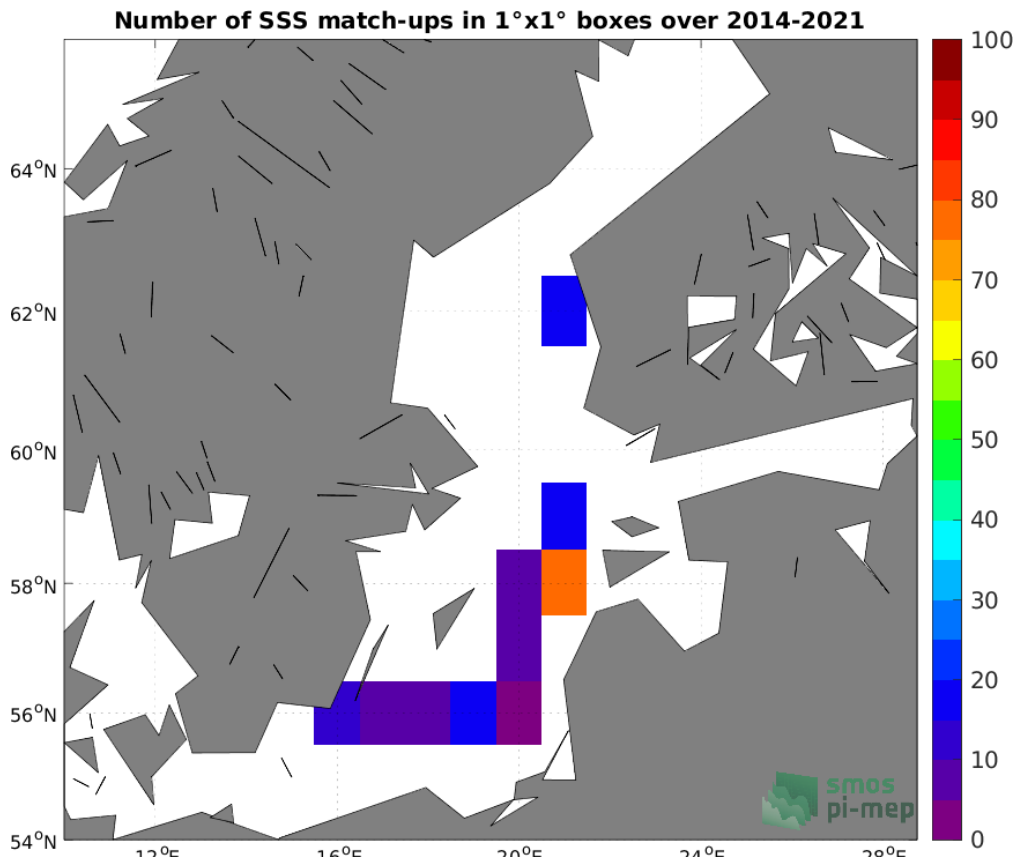
Figure 4: Number of SSS match-ups between Argo SSS and the SMOS SSS L3 v335 - Monthly - 25 km (CATDS-CPDC) SSS product for the Baltic Sea Pi-MEP region over 1°×1° boxes and for the full satellite product period.
