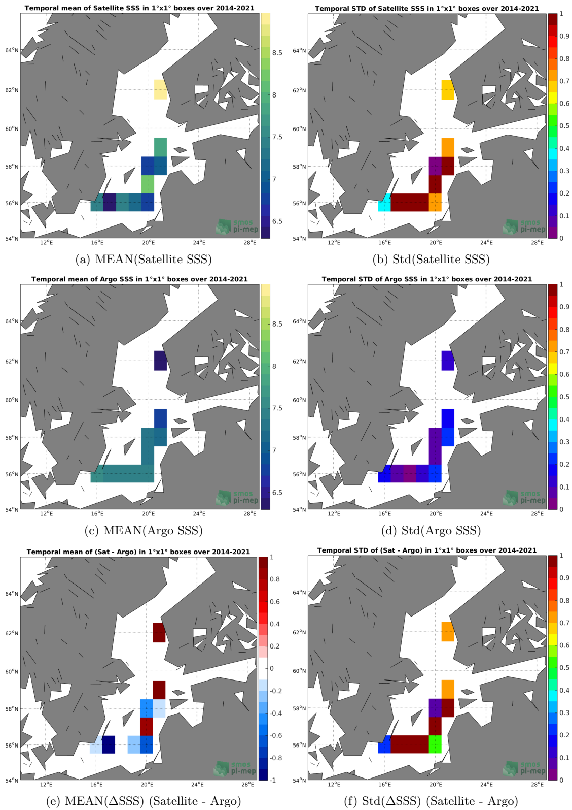
Figure 6: Temporal mean (left) and Std (right) of SSS from SMOS SSS L3 v335 - Monthly - 25 km (CATDS-CPDC) (top), Argo (middle), and \Delta SSS (Satellite - Argo). Only match-up pairs are used to generate these maps.
