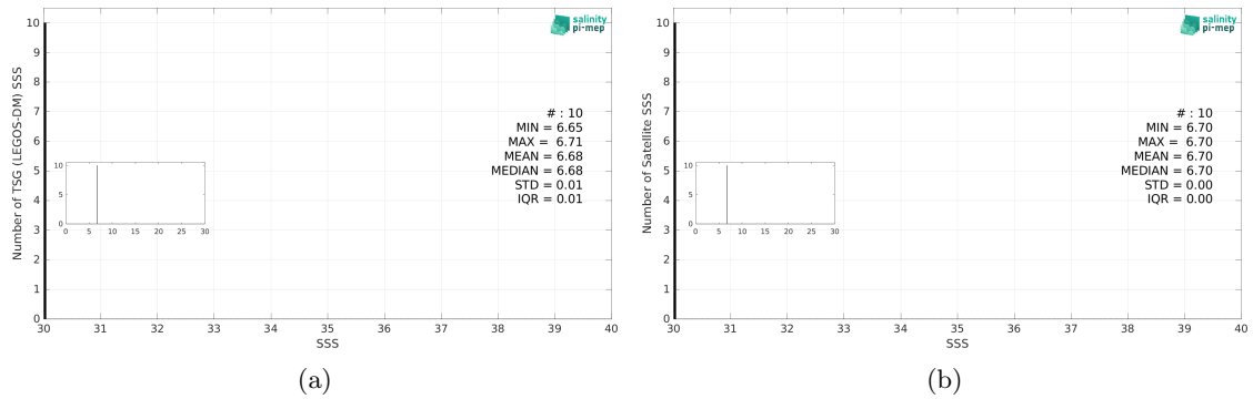
Figure 3: Histograms of SSS from TSG (LEGOS-DM) (a) and SMOS SSS L3 v335 - 10 Days - 25 km (CATDS-CPDC) (b) considering all match-up pairs per bins of 0.1 over the Baltic Sea Pi-MEP region and for the full satellite product period.
