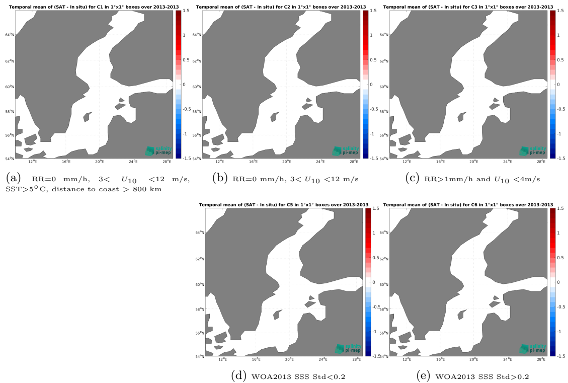
Figure 14: Temporal mean gridded over spatial boxes of size 1^\circ \times 1^\circ of \Delta SSS (SMOS SSS L3 v335 - 10 Days - 25 km (CATDS-CPDC) - TSG (LEGOS-DM)) for 5 different subdatasets corresponding to:RR=0 mm/h, 3 < U_{10} < 12 m/s, SST >5^\circ\text{C} , distance to coast > 800 km (a), RR=0 mm/h, 3 < U_{10} < 12 m/s (b), RR >1 mm/h and U_{10} < 4 m/s (c), WOA2013 SSS Std <0.2 (d), WOA2013 SSS Std >0.2 (e).
