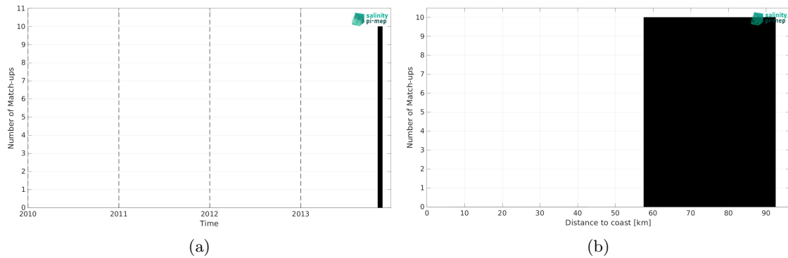
Figure 2: Number of match-ups between TSG (LEGOS-DM) and SMOS SSS L3 v335 - 10 Days - 25 km (CATDS-CPDC) SSS as a function of time (a) and as function of the distance to coast (b) over the Baltic Sea Pi-MEP region and for the full satellite product period.
