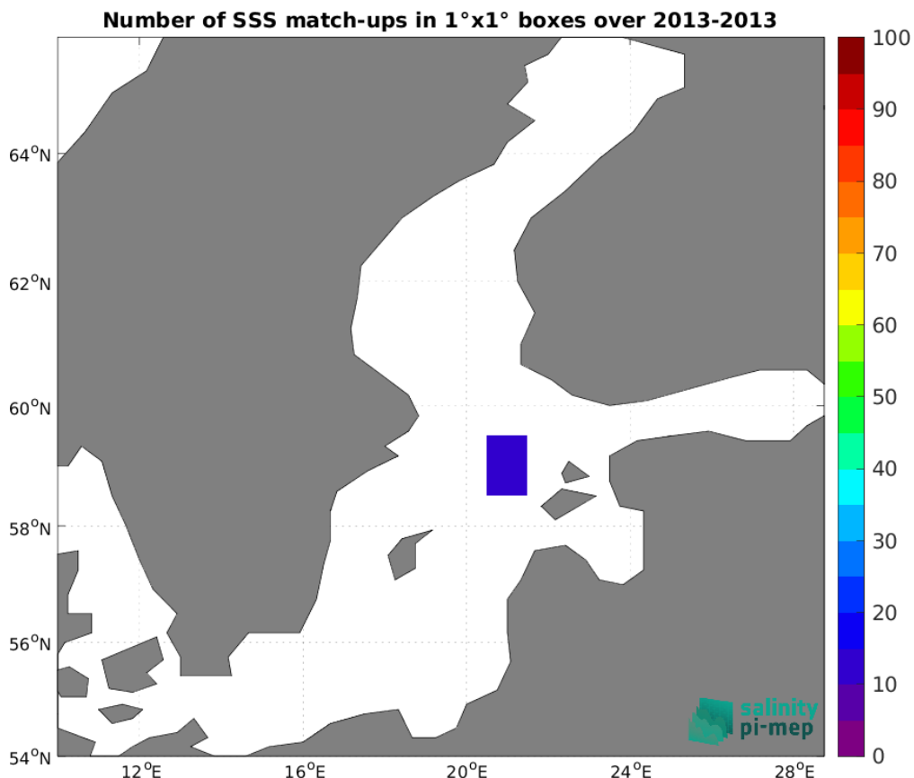
Figure 5: Number of SSS match-ups between TSG (LEGOS-DM) SSS and the SMOS SSS L3 v335 - 10 Days - 25 km (CATDS-CPDC) SSS product for the Baltic Sea Pi-MEP region over 1°x1° boxes and for the full satellite product period.
