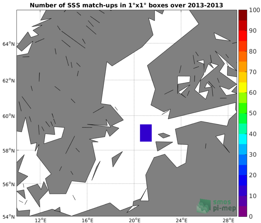
Figure 4: Number of SSS match-ups between TSG (LEGOS-DM) SSS and the SMOS SSS L3 v335 - 10 Days - 25 km (CATDS-CPDC) SSS product for the Baltic Sea Pi-MEP region over 1^\circ \times 1^\circ boxes and for the full satellite product period.
