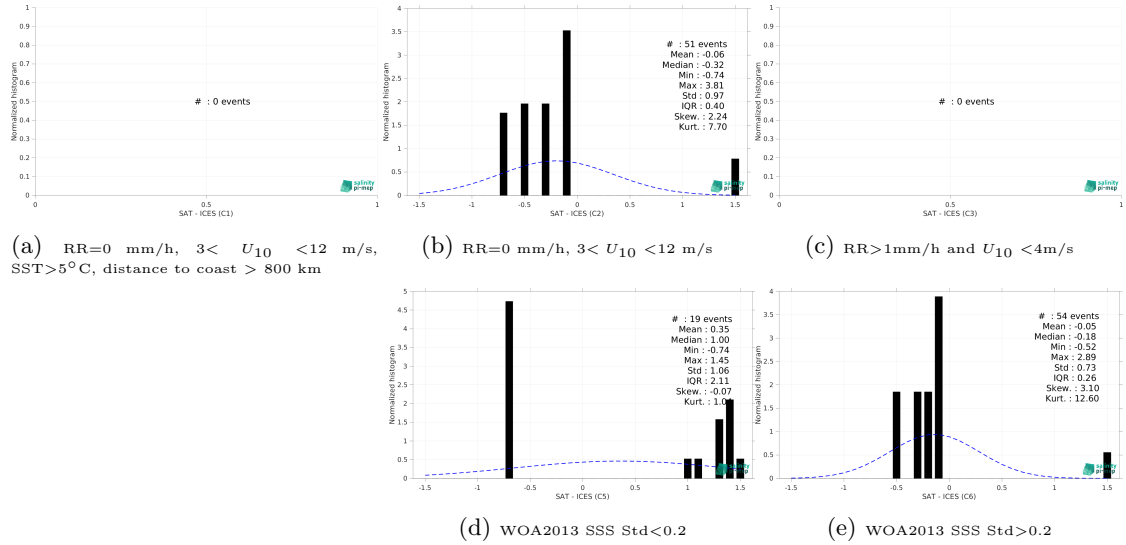
Figure 15: Normalized histogram of \Delta SSS (SMOS SSS L3 v335 - 10 Days - 25 km (CATDS-CPDC) - ICES) for 5 different subdatasets corresponding to: RR=0 mm/h, 3 < U_{10} < 12 m/s, SST>5°C, distance to coast > 800 km (a), RR=0 mm/h, 3 < U_{10} < 12 m/s (b), RR>1mm/h and U_{10} < 4 m/s (c), WOA2013 SSS Std<0.2 (d), WOA2013 SSS Std>0.2 (e).
