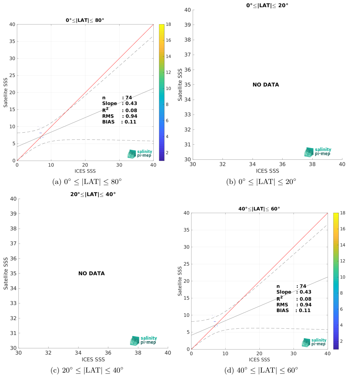
Figure 10: Contour maps of the concentration of SMOS SSS L3 v335 - 10 Days - 25 km (CATDS-CPDC) SSS (y-axis) versus ICES SSS (x-axis) at match-up pairs for different latitude bands. For each plot, the red line shows x=y . The black thin and dashed lines indicate a linear fit through the data cloud and the \pm 95\% confidence levels, respectively. The number match-up pairs n , the slope and R^2 coefficient of the linear fit, the root mean square (RMS) and the mean bias between satellite and in situ data are indicated for each latitude band in each plots.
