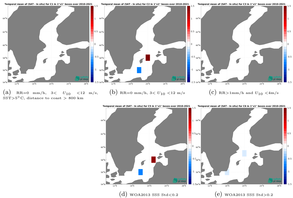
Figure 14: Temporal mean gridded over spatial boxes of size 1^\circ \times 1^\circ of \Delta SSS (SMOS SSS L3 v335 - 10 Days - 25 km (CATDS-CPDC) - ICES) for 5 different subdatasets corresponding to:RR=0 mm/h, 3 < U_{10} < 12 m/s, SST >5^\circ C, distance to coast > 800 km (a), RR=0 mm/h, 3 < U_{10} < 12 m/s (b), RR >1 mm/h and U_{10} < 4 m/s (c), WOA2013 SSS Std <0.2 (d), WOA2013 SSS Std >0.2 (e).
