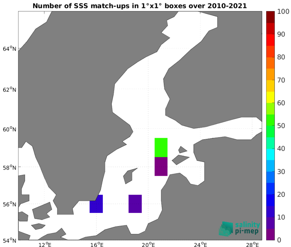
Figure 5: Number of SSS match-ups between ICES SSS and the SMOS SSS L3 v335 - 10 Days - 25 km (CATDS-CPDC) SSS product for the Baltic Sea Pi-MEP region over 1°x1° boxes and for the full satellite product period.
