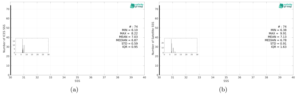
Figure 3: Histograms of SSS from ICES (a) and SMOS SSS L3 v335 - 10 Days - 25 km (CATDS-CPDC) (b) considering all match-up pairs per bins of 0.1 over the Baltic Sea Pi-MEP region and for the full satellite product period.
