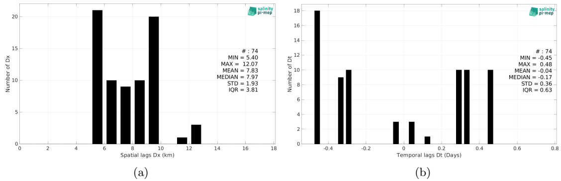
Figure 6: Histograms of the spatial (a) and temporal (b) lags between the location/time of the ICES measurement and the date of the corresponding SMOS SSS L3 v335 - 10 Days - 25 km (CATDS-CPDC) SSS pixel.
