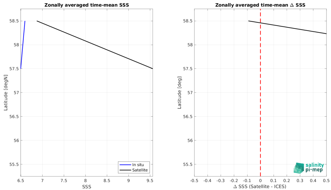
Figure 9: Left panel: Zonal mean SSS from SMOS SSS L3 v335 - 10 Days - 25 km (CATDS-CPDC) satellite product (black) and from ICES (blue). Right panel: Zonal mean of \Delta SSS (Satellite - ICES) for all the collected Pi-MEP match-up pairs estimated over the full satellite product period.
