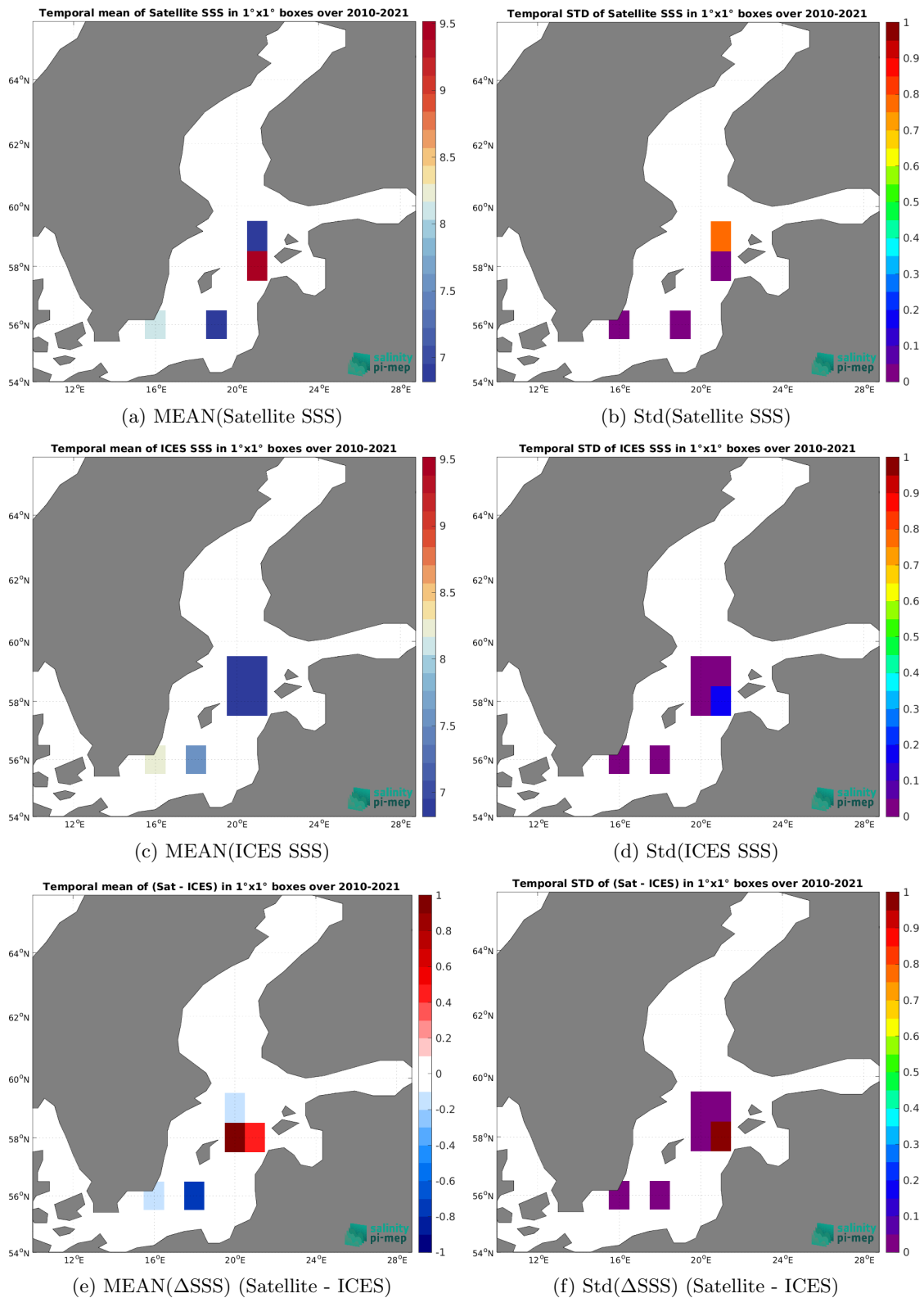
Figure 7: Temporal mean (left) and Std (right) of SSS from SMOS SSS L3 v335 - 10 Days - 25 km (CATDS-CPDC) (top), ICES (middle), and of \Delta SSS (Satellite - ICES). Only match-up pairs are used to generate these maps.
