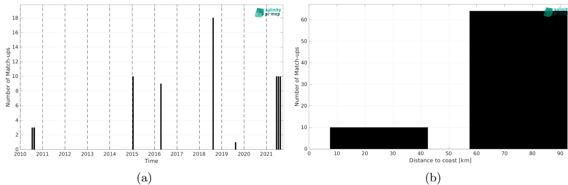
Figure 1: Number of match-ups between ICES and SMOS SSS L3 v335 - 10 Days - 25 km (CATDS-CPDC) SSS as a function of time (a) and as function of the distance to coast (b) over the Baltic Sea Pi-MEP region and for the full satellite product period.
