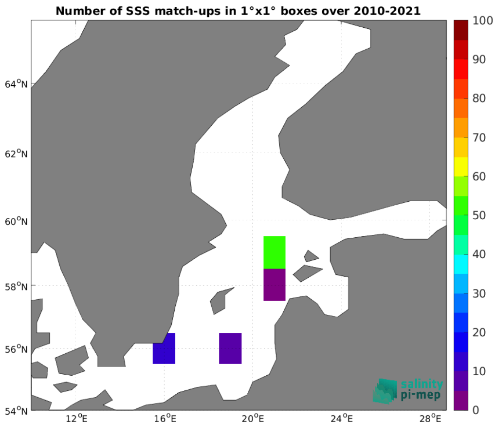
Figure 4: Number of SSS match-ups between ICES SSS and the SMOS SSS L3 v335 - 10 Days - 25 km (CATDS-CPDC) SSS product for the Baltic Sea Pi-MEP region over 1°x1° boxes and for the full satellite product period.
