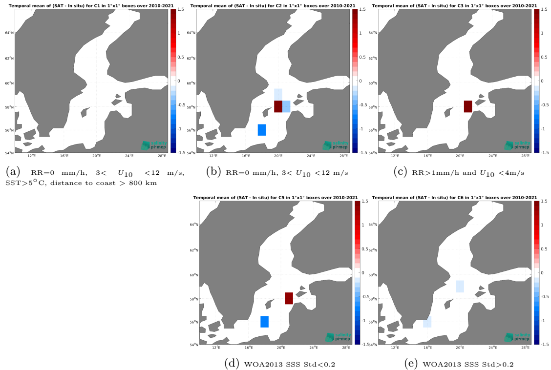
Figure 12: Temporal mean gridded over spatial boxes of size 1^{\circ}\times 1^{\circ} of \Delta\text{SSS} (SMOS SSS L3 v335 - 10 Days - 25 km (CATDS-CPDC) - ICES) for 5 different subdatasets corresponding to:RR=0 mm/h, 3 < U_{10} < 12 m/s, SST > 5^{\circ}\text{C} , distance to coast > 800 km (a), RR=0 mm/h, 3 < U_{10} < 12 m/s (b), RR > 1 mm/h and U_{10} < 4 m/s (c), WOA2013 SSS Std < 0.2 (d), WOA2013 SSS Std > 0.2 (e).
