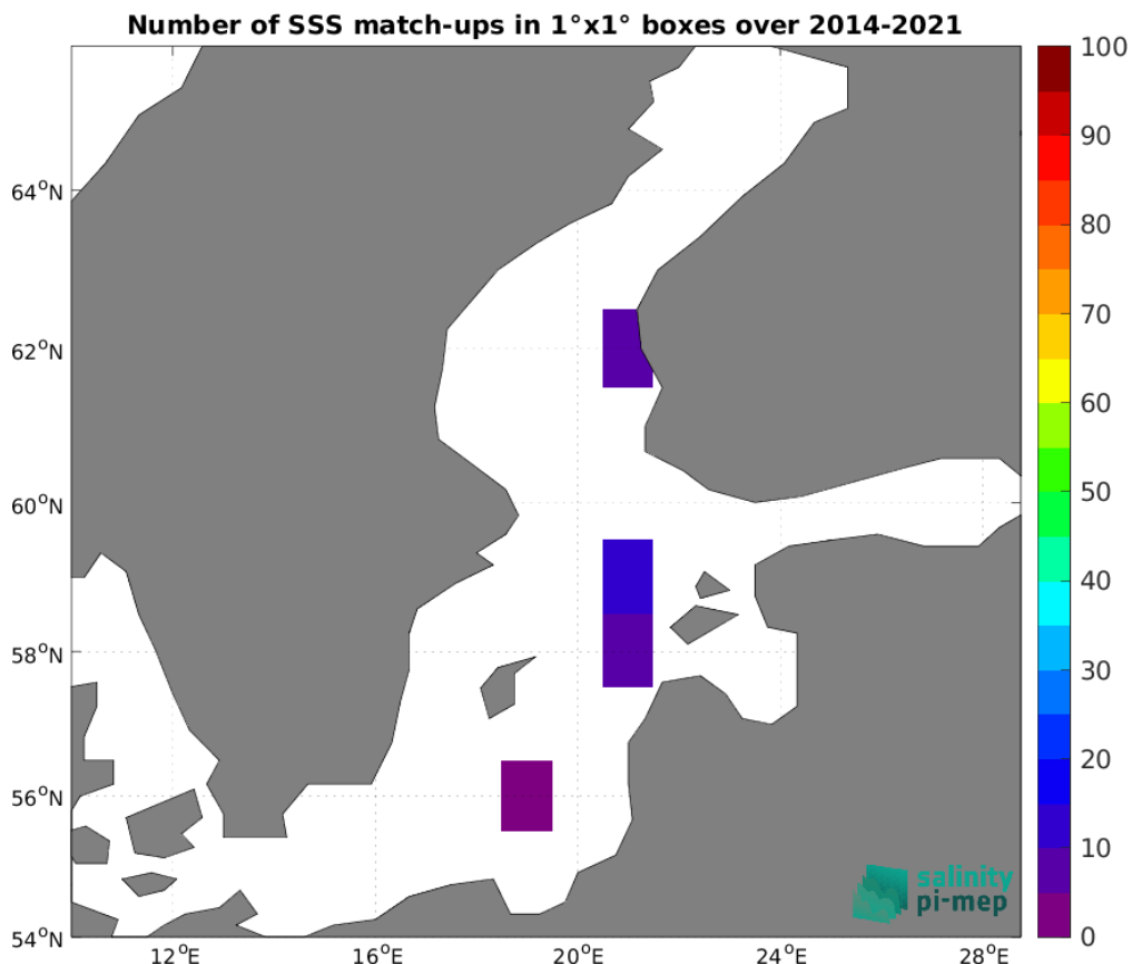
Figure 5: Number of SSS match-ups between Argo SSS and the SMOS SSS L3 v335 - 10 Days - 25 km (CATDS-CPDC) SSS product for the Baltic Sea Pi-MEP region over 1°x1° boxes and for the full satellite product period.
