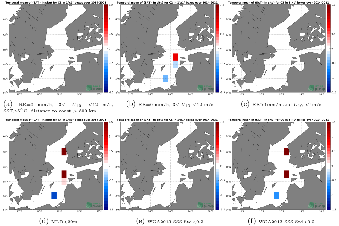
Figure 12: Temporal mean gridded over spatial boxes of size 1^{\circ} \times 1^{\circ} of \Delta\text{SSS} (SMOS SSS L3 v335 - 10 Days - 25 km (CATDS-CPDC) - Argo) for 6 different subdatasets corresponding to: RR=0 mm/h, 3 < U_{10} < 12 m/s, SST > 5^{\circ}\text{C} , distance to coast > 800 km (a), RR=0 mm/h, 3 < U_{10} < 12 m/s (b), RR > 1 mm/h and U_{10} < 4 m/s (c), MLD < 20\text{m} (d), WOA2013 SSS Std < 0.2 (e), WOA2013 SSS Std > 0.2 (f).
