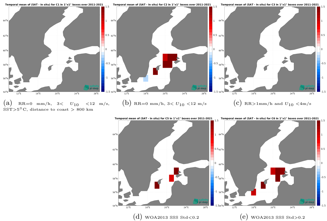
Figure 14: Temporal mean gridded over spatial boxes of size 1^\circ \times 1^\circ of \Delta SSS (SMOS SSS L3 v332 - 9 Days (CATDS-CPDC) - TSG (LEGOS-DM)) for 5 different subdatasets corresponding to:RR=0 mm/h, 3 < U_{10} < 12 m/s, SST >5^\circ\text{C} , distance to coast > 800 km (a), RR=0 mm/h, 3 < U_{10} < 12 m/s (b), RR >1 mm/h and U_{10} < 4 m/s (c), WOA2013 SSS Std <0.2 (d), WOA2013 SSS Std >0.2 (e).
