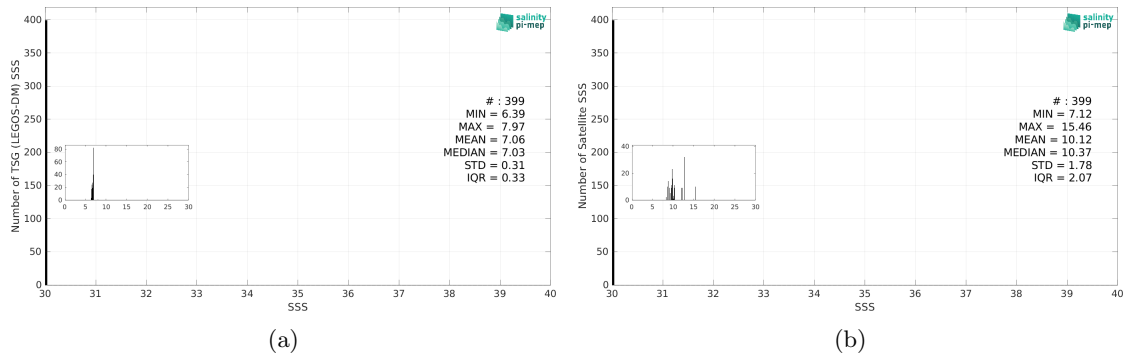
Figure 3: Histograms of SSS from TSG (LEGOS-DM) (a) and SMOS SSS L3 v332 - 9 Days (CATDS-CPDC) (b) considering all match-up pairs per bins of 0.1 over the Baltic Sea Pi-MEP region and for the full satellite product period.
