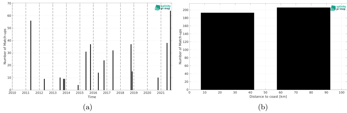
Figure 2: Number of match-ups between TSG (LEGOS-DM) and SMOS SSS L3 v332 - 9 Days (CATDS-CPDC) SSS as a function of time (a) and as function of the distance to coast (b) over the Baltic Sea Pi-MEP region and for the full satellite product period.
