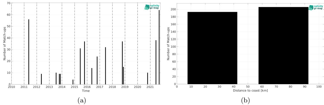
Figure 2: Number of match-ups between TSG (LEGOS-DM) and SMOS SSS L3 v332 - 9 Days (CATDS-CPDC) SSS as a function of time (a) and as function of the distance to coast (b) over the Baltic Sea Pi-MEP region and for the full satellite product period.
