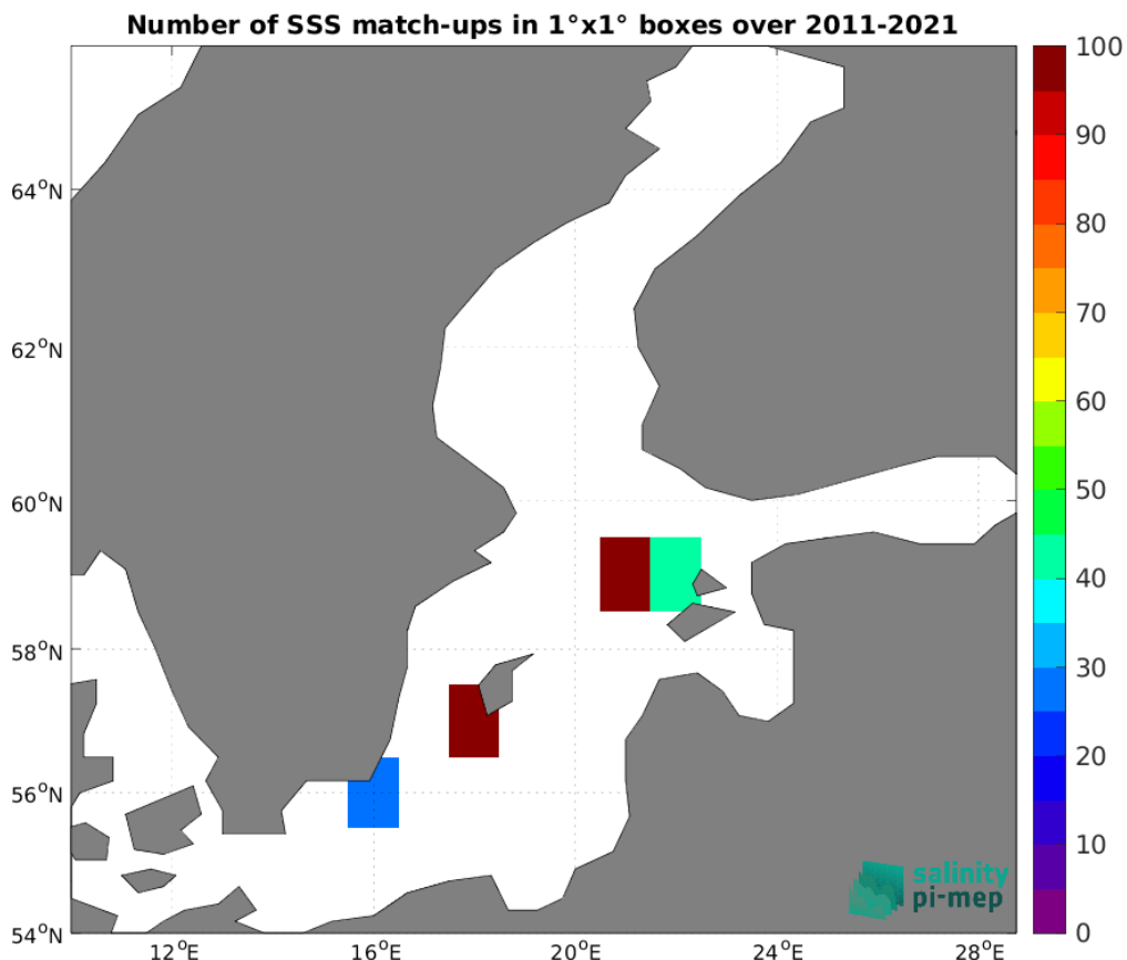
Figure 4: Number of SSS match-ups between TSG (LEGOS-DM) SSS and the SMOS SSS L3 v332 - 9 Days (CATDS-CPDC) SSS product for the Baltic Sea Pi-MEP region over 1°×1° boxes and for the full satellite product period.
