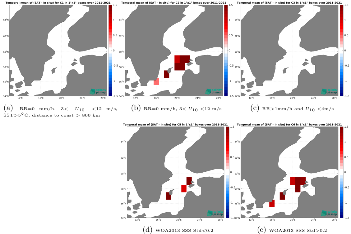
Figure 12: Temporal mean gridded over spatial boxes of size 1^{\circ}\times 1^{\circ} of \Delta\text{SSS} (SMOS SSS L3 v332 - 9 Days (CATDS-CPDC) - TSG (LEGOS-DM)) for 5 different subdatasets corresponding to:RR=0 mm/h, 3 < U_{10} < 12 m/s, SST >5^{\circ}\text{C} , distance to coast > 800 km (a), RR=0 mm/h, 3 < U_{10} < 12 m/s (b), RR >1 mm/h and U_{10} < 4 m/s (c), WOA2013 SSS Std <0.2 (d), WOA2013 SSS Std >0.2 (e).
