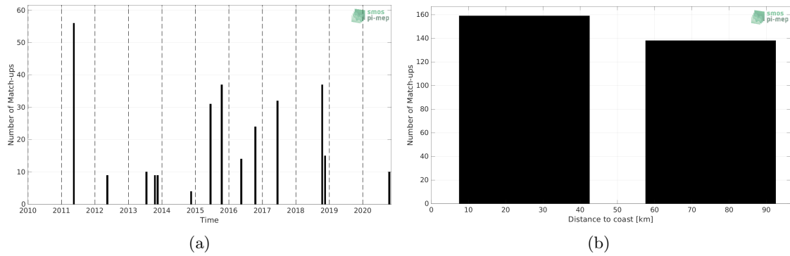
Figure 1: Number of match-ups between TSG (LEGOS-DM) and SMOS SSS L3 v332 - 9 Days (CATDS-CPDC) SSS as a function of time (a) and as function of the distance to coast (b) over the Baltic Sea Pi-MEP region and for the full satellite product period.
