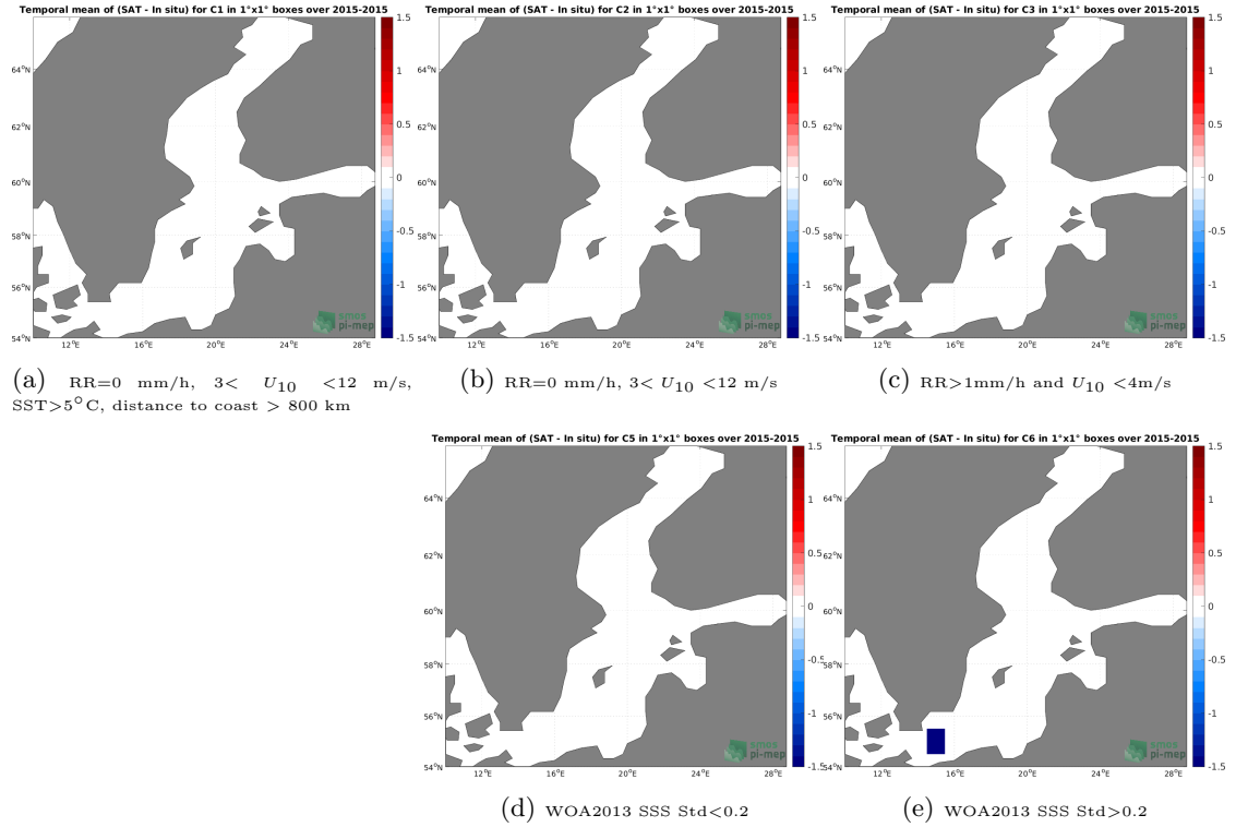
Figure 12: Temporal mean gridded over spatial boxes of size 1^{\circ}\times 1^{\circ} of \Delta SSS (SMOS SSS L3 v332 - 9 Days (CATDS-CPDC) - TSG (GOSUD-Research-vessel)) for 5 different subdatasets corresponding to:RR=0 mm/h, 3 < U_{10} < 12 m/s, SST >5^{\circ}\text{C} , distance to coast > 800 km (a), RR=0 mm/h, 3 < U_{10} < 12 m/s (b), RR >1 mm/h and U_{10} < 4 m/s (c), WOA2013 SSS Std <0.2 (d), WOA2013 SSS Std >0.2 (e).
