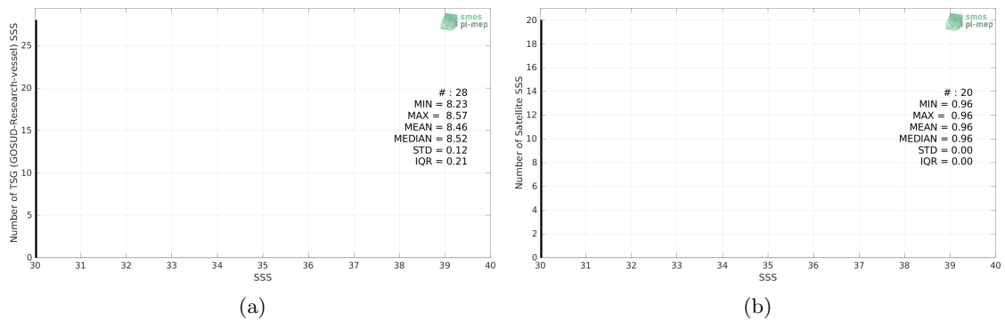
Figure 2: Histograms of SSS from TSG (GOSUD-Research-vessel) (a) and SMOS SSS L3 v332 - 9 Days (CATDS-CPDC) (b) considering all match-up pairs per bins of 0.1 over the Baltic Sea Pi-MEP region and for the full satellite product period.
