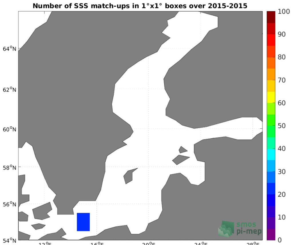
Figure 4: Number of SSS match-ups between TSG (GOSUD-Research-vessel) SSS and the SMOS SSS L3 v332 - 9 Days (CATDS-CPDC) SSS product for the Baltic Sea Pi-MEP region over 1°x1° boxes and for the full satellite product period.
