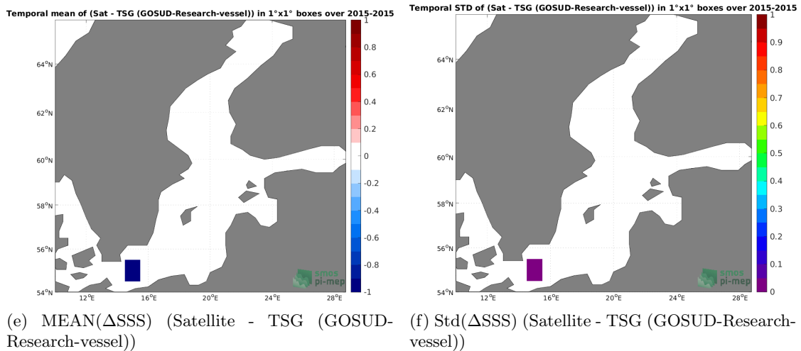
Figure 6: Temporal mean (left) and Std (right) of SSS from SMOS SSS L3 v332 - 9 Days (CATDS-CPDC) (top), TSG (GOSUD-Research-vessel) (middle), and of \Delta SSS (Satellite - TSG (GOSUD-Research-vessel)). Only match-up pairs are used to generate these maps.
