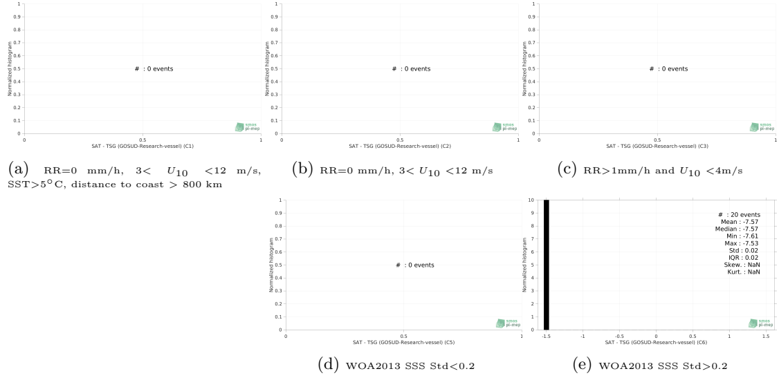
Figure 13: Normalized histogram of \Delta\text{SSS} (SMOS SSS L3 v332 - 9 Days (CATDS-CPDC) - TSG (GOSUD-Research-vessel)) for 5 different subdatasets corresponding to: RR=0 mm/h, 3 < U_{10} < 12 m/s, SST > 5^\circ\text{C} , distance to coast > 800 km (a), RR=0 mm/h, 3 < U_{10} < 12 m/s (b), RR > 1\text{mm/h} and U_{10} < 4\text{m/s} (c), WOA2013 SSS Std < 0.2 (d), WOA2013 SSS Std > 0.2 (e).
