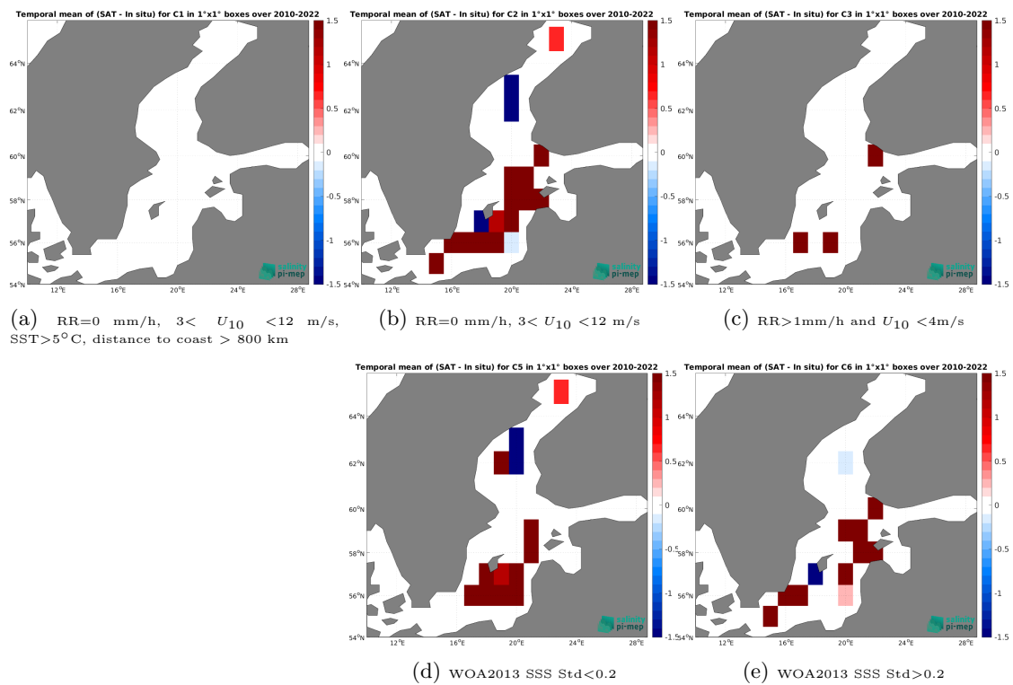
Figure 14: Temporal mean gridded over spatial boxes of size 1^\circ \times 1^\circ of \Delta\text{SSS} (SMOS SSS L3 v332 - 9 Days (CATDS-CPDC) - ICES) for 5 different subdatasets corresponding to: RR=0 mm/h, 3 < U_{10} < 12 m/s, SST > 5°C, distance to coast > 800 km (a), RR=0 mm/h, 3 < U_{10} < 12 m/s (b), RR > 1mm/h and U_{10} < 4 m/s (c), WOA2013 SSS Std < 0.2 (d), WOA2013 SSS Std > 0.2 (e).
