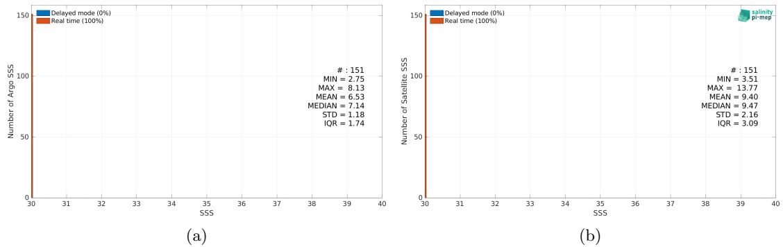
Figure 2: Histograms of SSS from Argo (a) and SMOS SSS L3 v332 - 9 Days (CATDS-CPDC) (b) considering all match-up pairs per bins of 0.1 over the Baltic Sea Pi-MEP region and for the full satellite product period.
