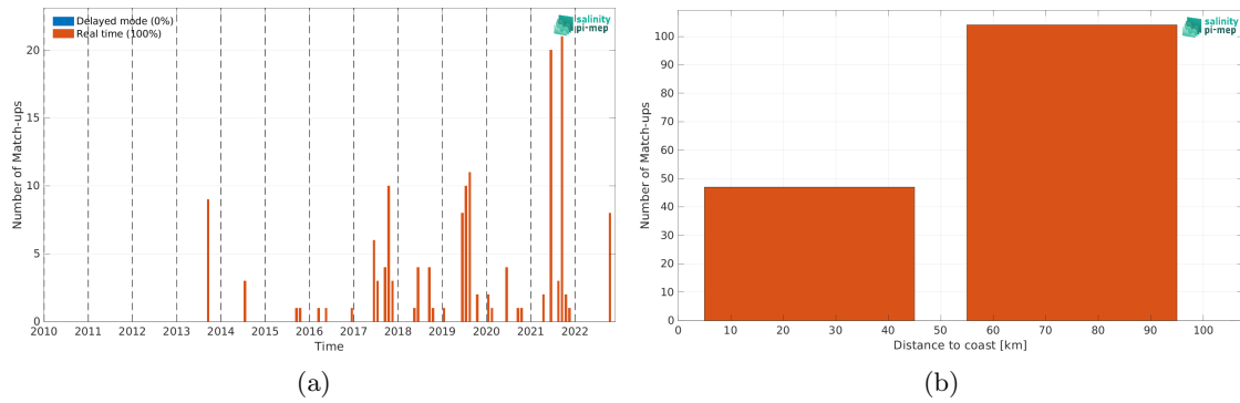
Figure 1: Number of match-ups between Argo and SMOS SSS L3 v332 - 9 Days (CATDS-CPDC) SSS as a function of time (a) and as function of the distance to coast (b) over the Baltic Sea Pi-MEP region and for the full satellite product period.
