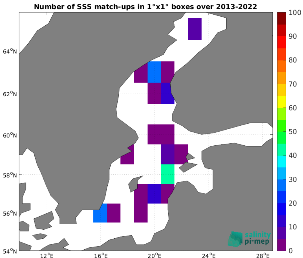
Figure 4: Number of SSS match-ups between Argo SSS and the SMOS SSS L3 v332 - 9 Days (CATDS-CPDC) SSS product for the Baltic Sea Pi-MEP region over 1°x1° boxes and for the full satellite product period.
