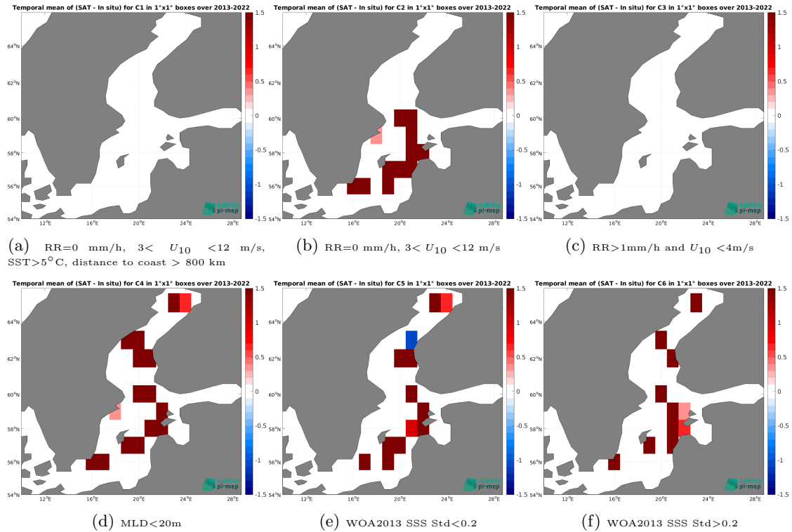
Figure 12: Temporal mean gridded over spatial boxes of size 1^{\circ}\times 1^{\circ} of \Delta\text{SSS} (SMOS SSS L3 v332 - 9 Days (CATDS-CPDC) - Argo) for 6 different subdatasets corresponding to:RR=0 mm/h, 3 < U_{10} < 12 m/s, SST >5^{\circ}\text{C} , distance to coast > 800 km (a), RR=0 mm/h, 3 < U_{10} < 12 m/s (b), RR >1\text{mm/h} and U_{10} < 4\text{m/s} (c),MLD <20\text{m} (d),WOA2013 SSS Std <0.2 (e),WOA2013 SSS Std >0.2 (f).
