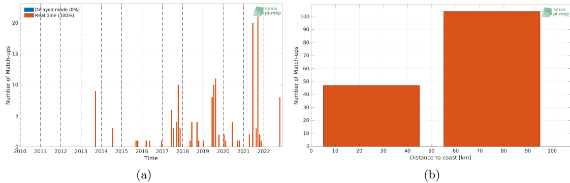
Figure 1: Number of match-ups between Argo and SMOS SSS L3 v332 - 9 Days (CATDS-CPDC) SSS as a function of time (a) and as function of the distance to coast (b) over the Baltic Sea Pi-MEP region and for the full satellite product period.
