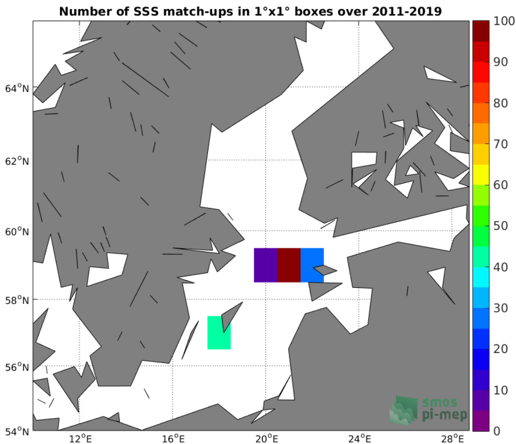
Figure 4: Number of SSS match-ups between TSG (LEGOS-DM) SSS and the SMOS SSS L3 v317 - Monthly - 25 km (CATDS-CPDC) SSS product for the Baltic Sea Pi-MEP region over 1^\circ \times 1^\circ boxes and for the full satellite product period.
