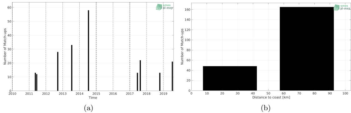
Figure 1: Number of match-ups between TSG (LEGOS-DM) and SMOS SSS L3 v317 - Monthly - 25 km (CATDS-CPDC) SSS as a function of time (a) and as function of the distance to coast (b) over the Baltic Sea Pi-MEP region and for the full satellite product period.
