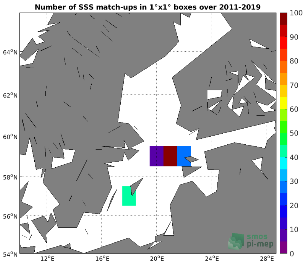
Figure 4: Number of SSS match-ups between TSG (LEGOS-DM) SSS and the SMOS SSS L3 v317 - Monthly - 25 km (CATDS-CPDC) SSS product for the Baltic Sea Pi-MEP region over 1°x1° boxes and for the full satellite product period.
