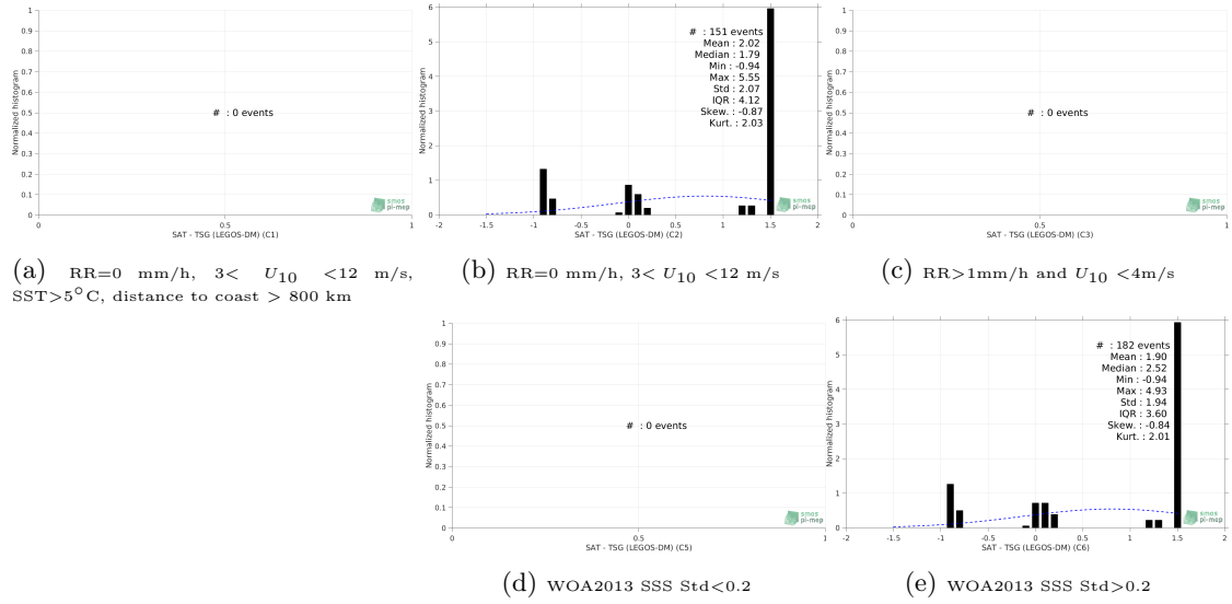
Figure 13: Normalized histogram of \Delta\text{SSS} (SMOS SSS L3 v317 - Monthly - 25 km (CATDS-CPDC) - TSG (LEGOS-DM)) for 5 different subdatasets corresponding to: RR=0 mm/h, 3 < U_{10} < 12 m/s, SST > 5^\circ\text{C} , distance to coast > 800 km (a), RR=0 mm/h, 3 < U_{10} < 12 m/s (b), RR > 1\text{mm/h} and U_{10} < 4\text{m/s} (c), WOA2013 SSS Std < 0.2 (d), WOA2013 SSS Std > 0.2 (e).
