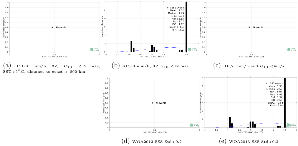
Figure 13: Normalized histogram of \Delta SSS (SMOS L3 v317 - Monthly - 25 km (CATDS-CPDC) - TSG-LEGOS-DM) for 5 different subdatasets corresponding to: RR=0 mm/h, 3 < U_{10} < 12 m/s, SST > 5°C, distance to coast > 800 km (a), RR=0 mm/h, 3 < U_{10} < 12 m/s (b), RR > 1mm/h and U_{10} < 4 m/s (c), WOA2013 SSS Std < 0.2 (d), WOA2013 SSS Std > 0.2 (e).
