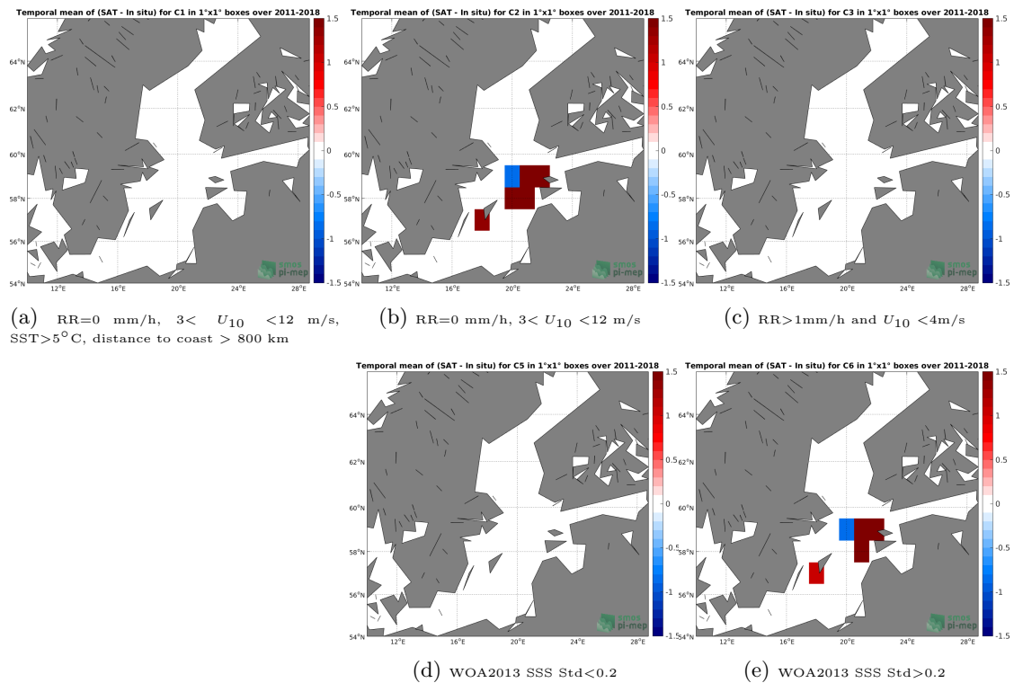
Figure 12: Temporal mean gridded over spatial boxes of size 1^{\circ}\times 1^{\circ} of \Delta\text{SSS} (SMOS L3 v317 - Monthly - 25 km (CATDS-CPDC) - TSG-LEGOS-DM) for 5 different subdatasets corresponding to: \text{RR}=0 mm/h, 3 < U_{10} < 12 m/s, \text{SST} > 5^{\circ}\text{C} , distance to coast > 800 km (a), \text{RR}=0 mm/h, 3 < U_{10} < 12 m/s (b), \text{RR} > 1 mm/h and U_{10} < 4 m/s (c), WOA2013 SSS Std < 0.2 (d), WOA2013 SSS Std > 0.2 (e).
