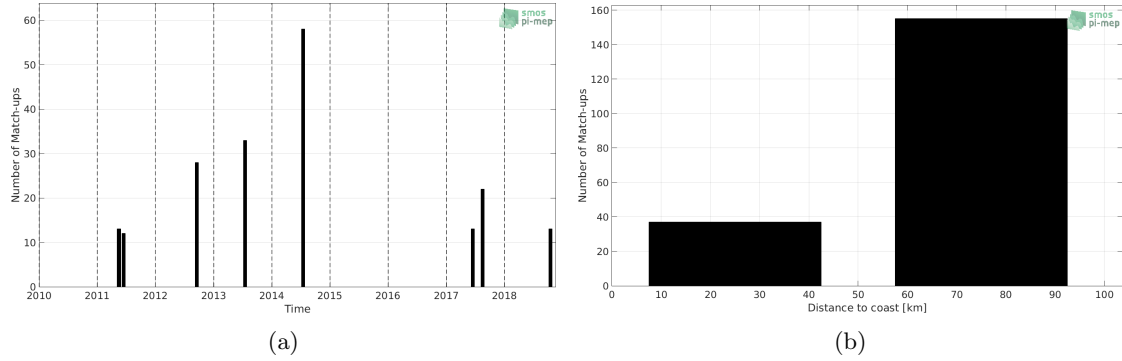
Figure 1: Number of match-ups between TSG-LEGOS-DM and SMOS L3 v317 - Monthly - 25 km (CATDS-CPDC) SSS as a function of time (a) and as function of the distance to coast (b) over the Baltic Sea Pi-MEP region and for the full satellite product period.
