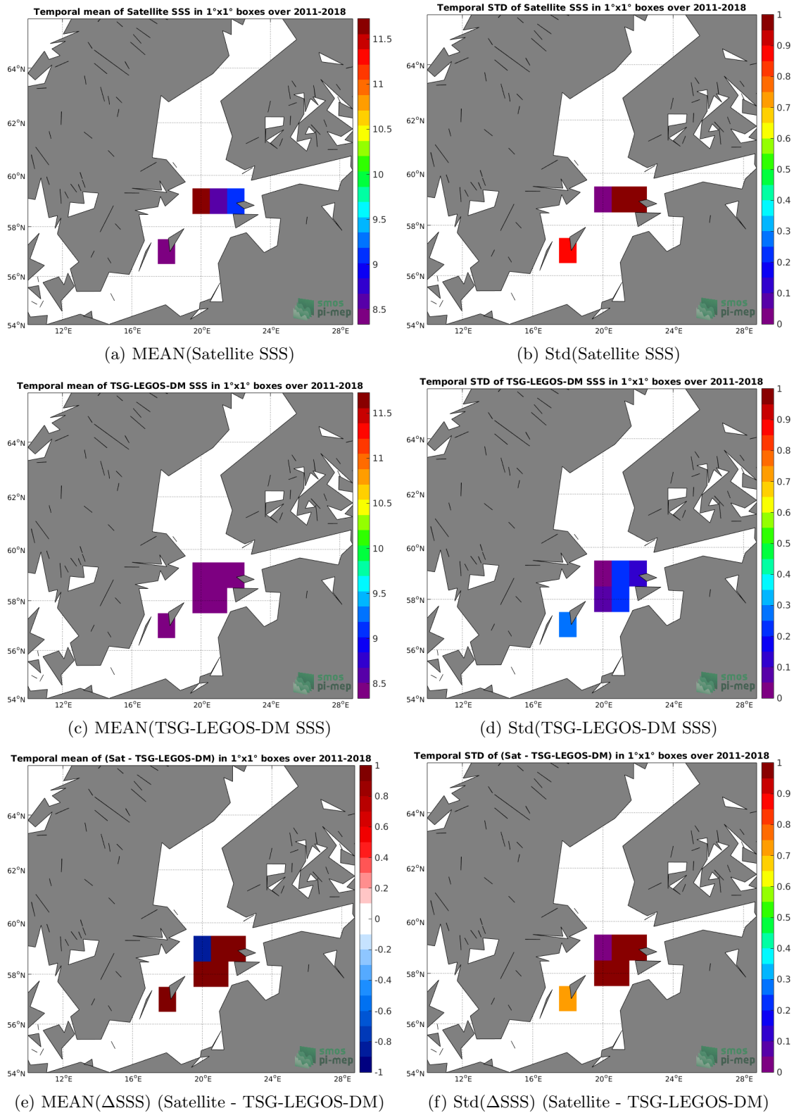
Figure 6: Temporal mean (left) and Std (right) of SSS from SMOS L3 v317 - Monthly - 25 km (CATDS-CPDC) (top), TSG-LEGOS-DM (middle), and of \Delta SSS (Satellite - TSG-LEGOS-DM). Only match-up pairs are used to generate these maps.
