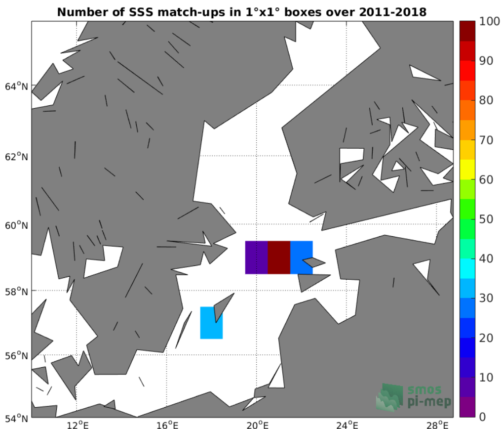
Figure 4: Number of SSS match-ups between TSG-LEGOS-DM SSS and the SMOS L3 v317 - Monthly - 25 km (CATDS-CPDC) SSS product for the Baltic Sea Pi-MEP region over 1°x1° boxes and for the full satellite product period.
