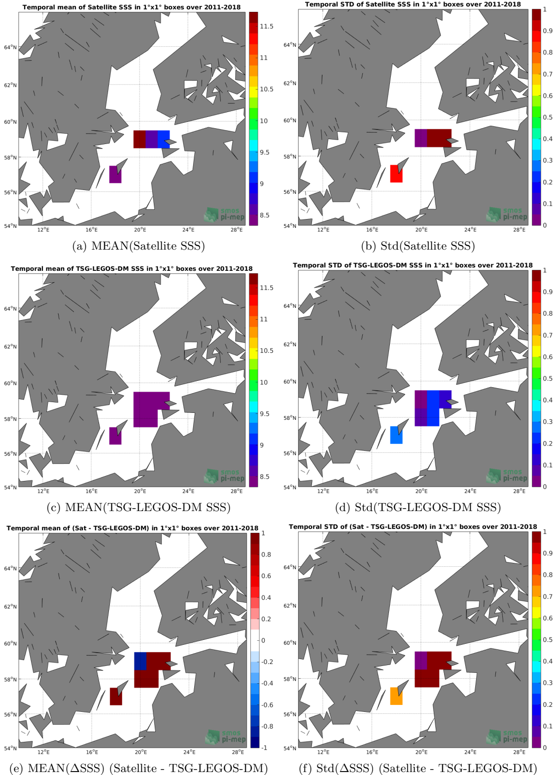
Figure 6: Temporal mean (left) and Std (right) of SSS from SMOS-L3-CATDS-CPDC-V317-MONTHLY-25KM (top), TSG-LEGOS-DM (middle), and of \Delta SSS (Satellite - TSG-LEGOS-DM). Only match-up pairs are used to generate these maps.
