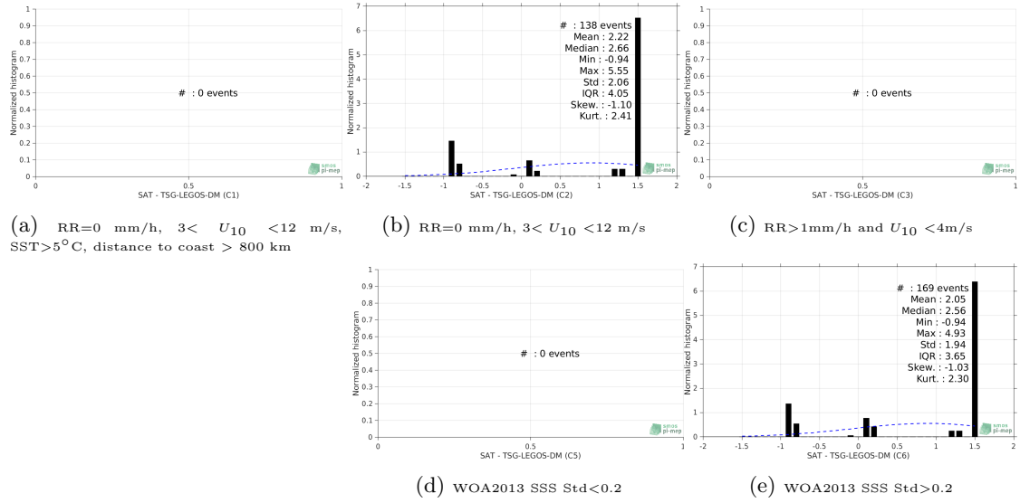
Figure 13: Normalized histogram of \Delta\text{SSS} (SMOS-L3-CATDS-CPDC-V317-MONTHLY-25KM - TSG-LEGOS-DM) for 5 different subdatasets corresponding to: RR=0 mm/h, 3 < U_{10} < 12 m/s, SST > 5^{\circ}\text{C} , distance to coast > 800 km (a), RR=0 mm/h, 3 < U_{10} < 12 m/s (b), RR > 1\text{mm/h} and U_{10} < 4\text{m/s} (c), WOA2013 SSS Std < 0.2 (d), WOA2013 SSS Std > 0.2 (e).
