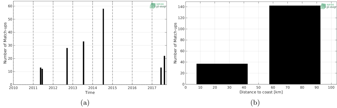
Figure 1: Number of match-ups between TSG-LEGOS-DM and SMOS-L3-CATDS-CPDC-V317-MONTHLY-25KM SSS as a function of time (a) and as function of the distance to coast (b) over the Baltic Sea Pi-MEP region and for the full satellite product period.
