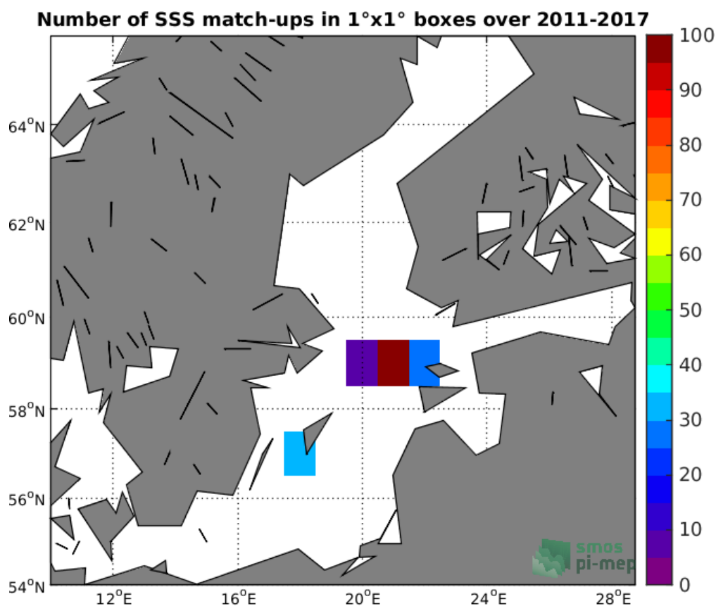
Figure 4: Number of SSS match-ups between TSG-LEGOS-DM SSS and the SMOS-L3-CATDS-CPDC-V317-MONTHLY-25KM SSS product for the Baltic Sea Pi-MEP region over 1°x1° boxes and for the full satellite product period.
