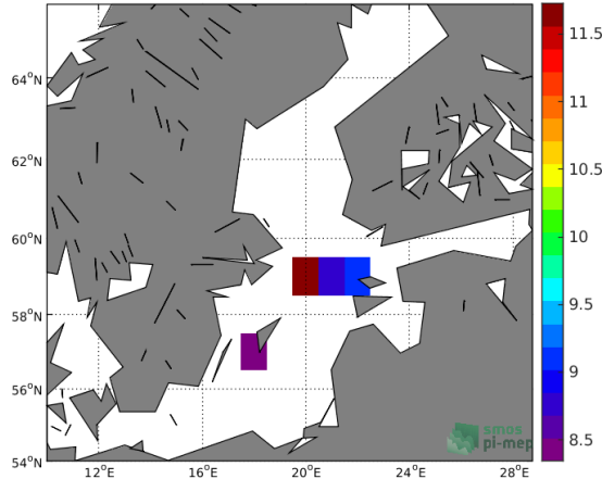
(a) MEAN(Satellite SSS)
