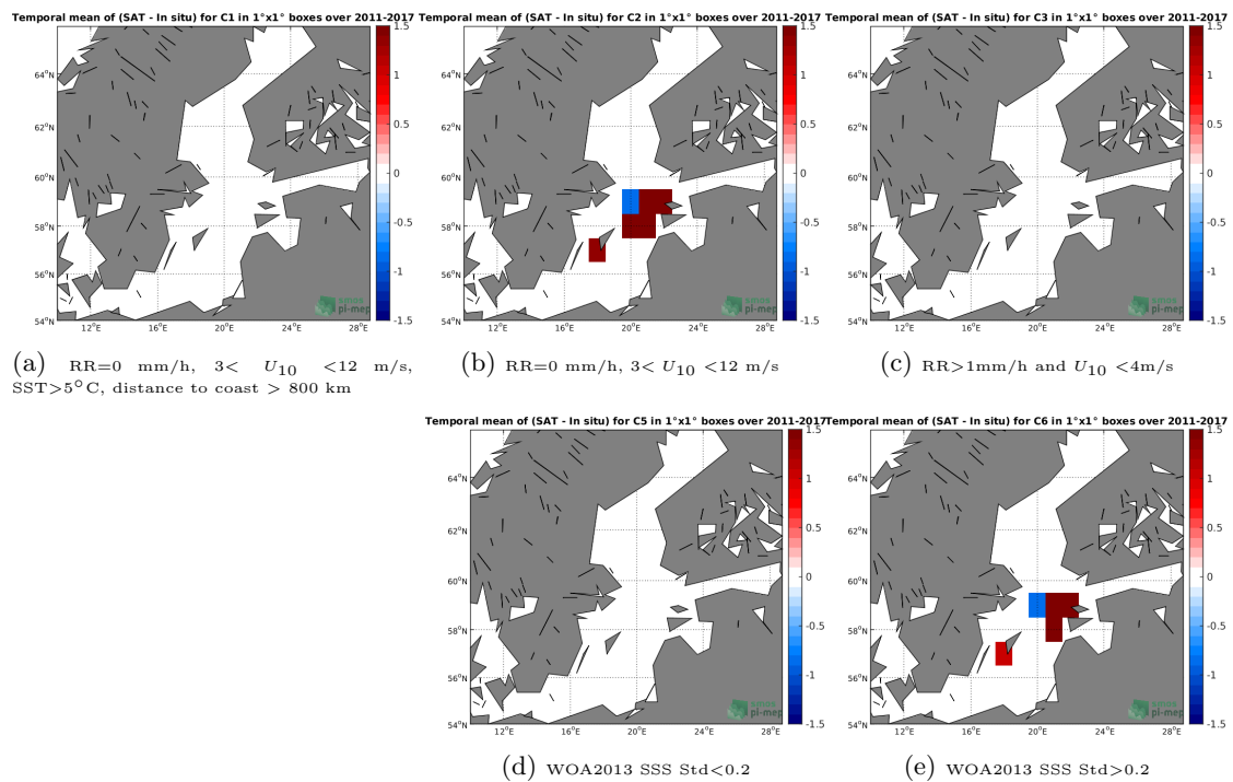
Figure 12: Temporal mean gridded over spatial boxes of size 1^\circ \times 1^\circ of \Delta SSS (SMOS-L3-CATDS-CPDC-V317-MONTHLY-25KM - TSG-LEGOS-DM) for 5 different subdatasets corresponding to: RR=0 mm/h, 3 < U_{10} < 12 m/s, SST > 5^\circ\text{C} , distance to coast > 800 km (a), RR=0 mm/h, 3 < U_{10} < 12 m/s (b), RR > 1 mm/h and U_{10} < 4 m/s (c), WOA2013 SSS Std < 0.2 (d), WOA2013 SSS Std > 0.2 (e).
