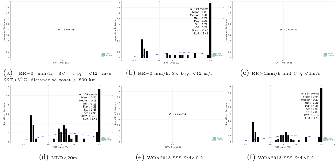
Figure 13: Normalized histogram of \Delta\text{SSS} (SMOS SSS L3 v317 - Monthly - 25 km (CATDS-CPDC) - Argo) for 6 different subdatasets corresponding to: RR=0 mm/h, 3 < U_{10} < 12 m/s, SST > 5^{\circ}\text{C} , distance to coast > 800 km (a), RR=0 mm/h, 3 < U_{10} < 12 m/s (b), RR > 1 mm/h and U_{10} < 4 m/s (c), MLD < 20 m (d), WOA2013 SSS Std < 0.2 (e), WOA2013 SSS Std > 0.2 (f).
