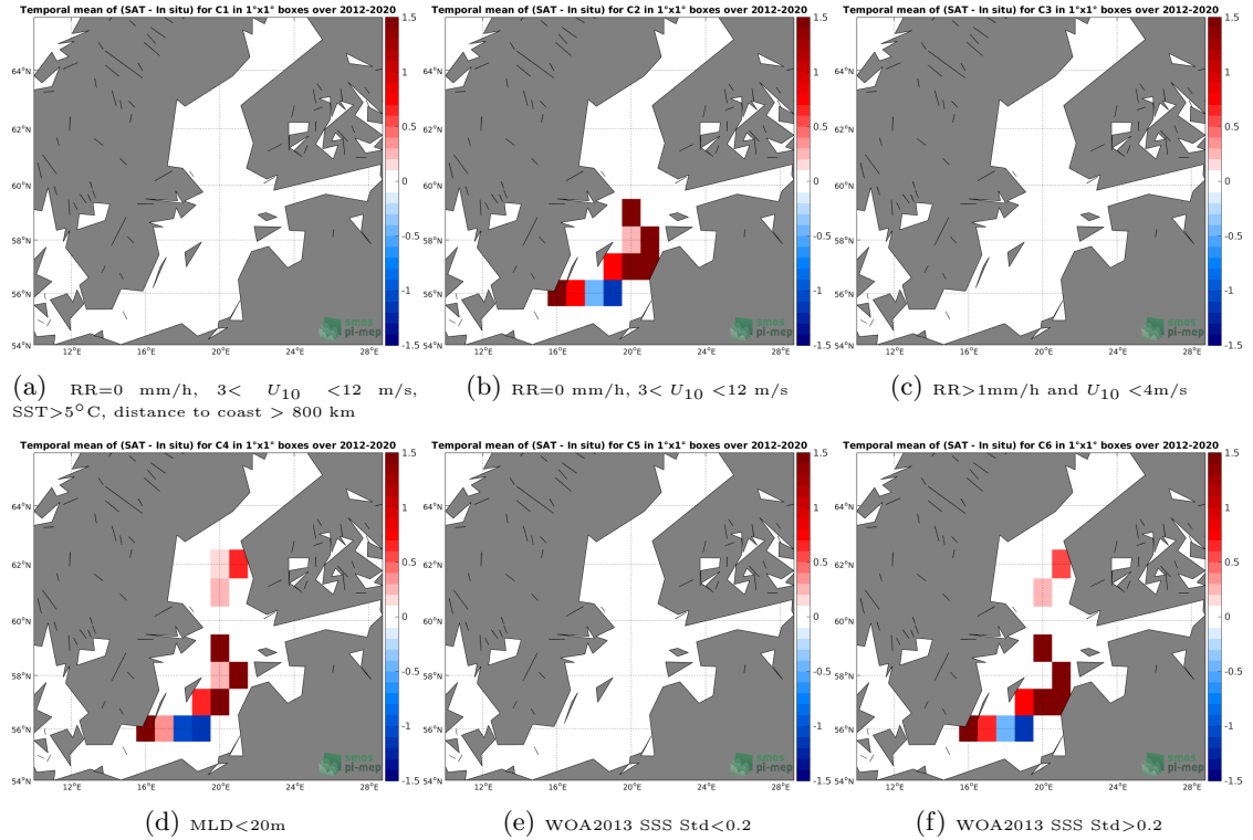
Figure 12: Temporal mean gridded over spatial boxes of size 1^{\circ} \times 1^{\circ} of \Delta\text{SSS} (SMOS SSS L3 v317 - Monthly - 25 km (CATDS-CPDC) - Argo) for 6 different subdatasets corresponding to: RR=0 mm/h, 3 < U_{10} < 12 m/s, SST >5^{\circ}\text{C} , distance to coast > 800 km (a), RR=0 mm/h, 3 < U_{10} < 12 m/s (b), RR >1 mm/h and U_{10} < 4 m/s (c),MLD <20 m (d),WOA2013 SSS Std <0.2 (e),WOA2013 SSS Std >0.2 (f).
