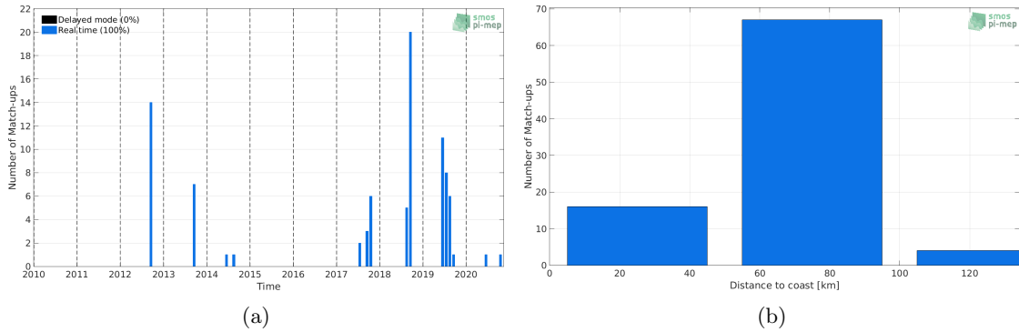
Figure 1: Number of match-ups between Argo and SMOS SSS L3 v317 - Monthly - 25 km (CATDS-CPDC) SSS as a function of time (a) and as function of the distance to coast (b) over the Baltic Sea Pi-MEP region and for the full satellite product period.
