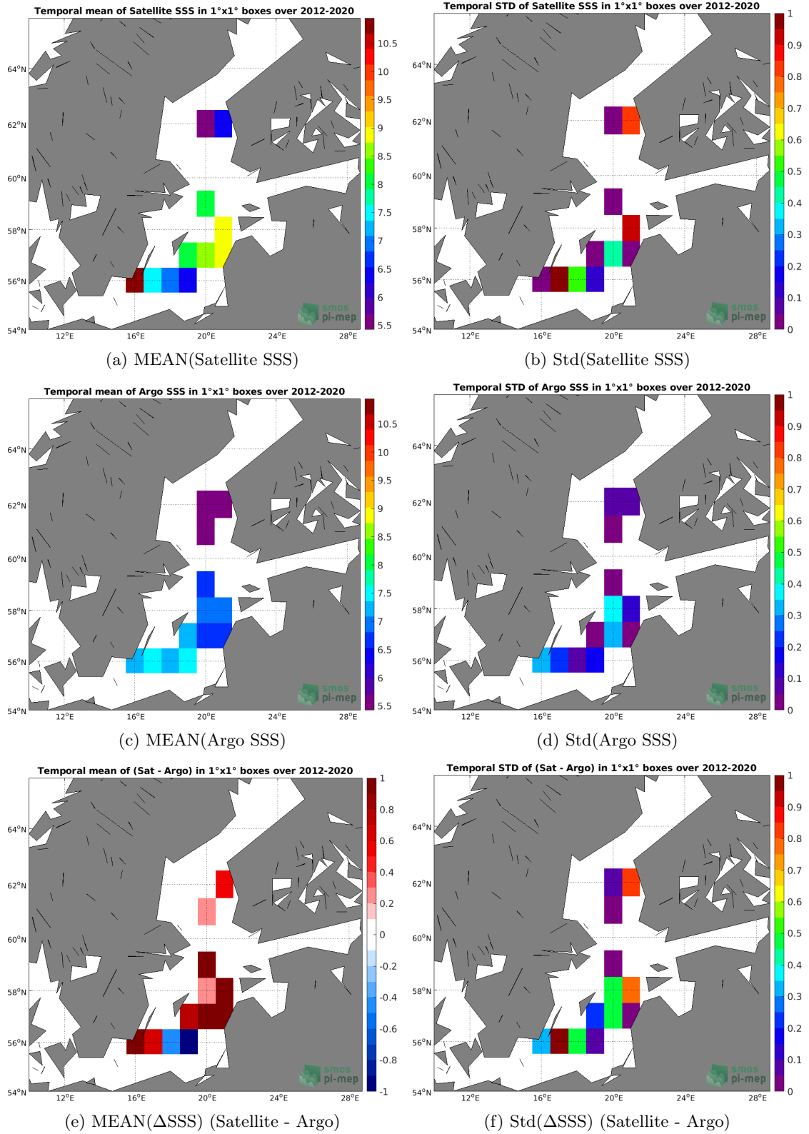
Figure 6: Temporal mean (left) and Std (right) of SSS from SMOS SSS L3 v317 - Monthly - 25 km (CATDS-CPDC) (top), Argo (middle), and \Delta SSS (Satellite - Argo). Only match-up pairs are used to generate these maps.
