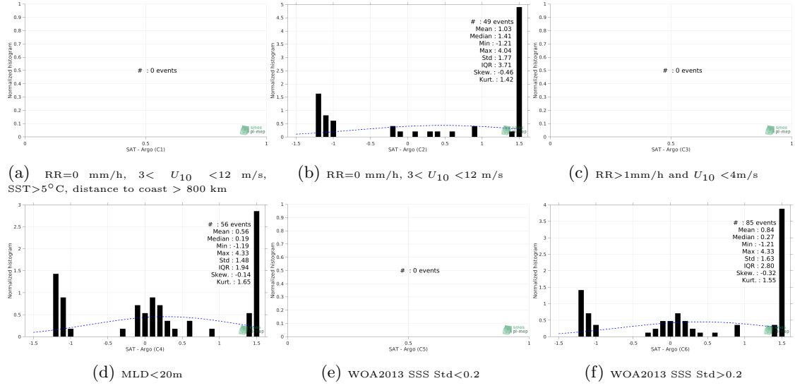
Figure 13: Normalized histogram of \Delta\text{SSS} (SMOS SSS L3 v317 - Monthly - 25 km (CATDS-CPDC) - Argo) for 6 different subdatasets corresponding to: RR=0 mm/h, 3 < U_{10} < 12 m/s, SST > 5^\circ\text{C} , distance to coast > 800 km (a), RR=0 mm/h, 3 < U_{10} < 12 m/s (b), RR > 1 mm/h and U_{10} < 4 m/s (c), MLD < 20 m (d), WOA2013 SSS Std < 0.2 (e), WOA2013 SSS Std > 0.2 (f).
