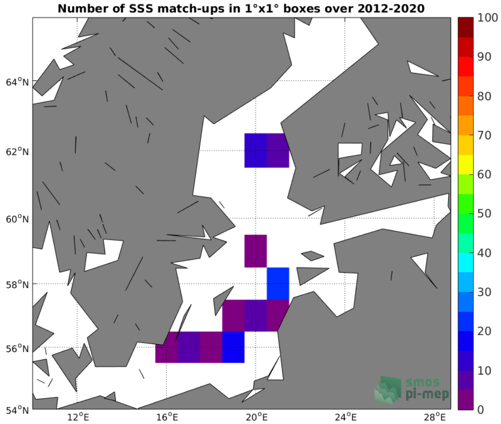
Figure 4: Number of SSS match-ups between Argo SSS and the SMOS SSS L3 v317 - Monthly - 25 km (CATDS-CPDC) SSS product for the Baltic Sea Pi-MEP region over 1°x1° boxes and for the full satellite product period.
