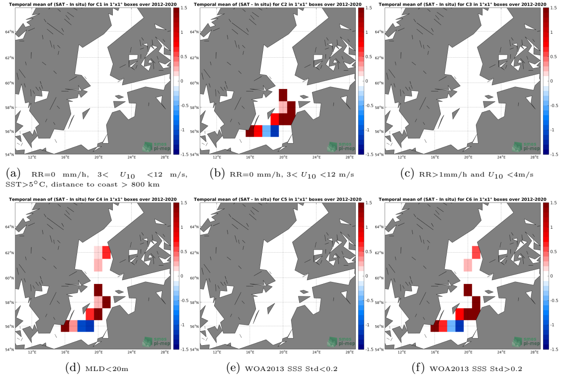
Figure 12: Temporal mean gridded over spatial boxes of size 1^{\circ}\times 1^{\circ} of \Delta\text{SSS} (SMOS SSS L3 v317 - Monthly - 25 km (CATDS-CPDC) - Argo) for 6 different subdatasets corresponding to: RR=0 mm/h, 3 < U_{10} < 12 m/s, SST > 5^{\circ}\text{C} , distance to coast > 800 km (a), RR=0 mm/h, 3 < U_{10} < 12 m/s (b), RR > 1 mm/h and U_{10} < 4 m/s (c), MLD < 20\text{m} (d), WOA2013 SSS Std < 0.2 (e), WOA2013 SSS Std > 0.2 (f).
