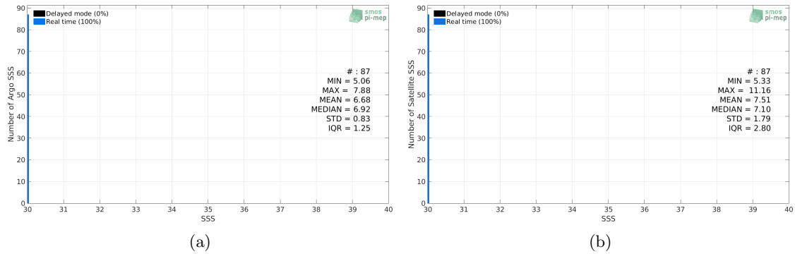
Figure 2: Histograms of SSS from Argo (a) and SMOS SSS L3 v317 - Monthly - 25 km (CATDS-CPDC) (b) considering all match-up pairs per bins of 0.1 over the Baltic Sea Pi-MEP region and for the full satellite product period.
