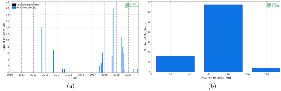
Figure 1: Number of match-ups between Argo and SMOS SSS L3 v317 - Monthly - 25 km (CATDS-CPDC) SSS as a function of time (a) and as function of the distance to coast (b) over the Baltic Sea Pi-MEP region and for the full satellite product period.
