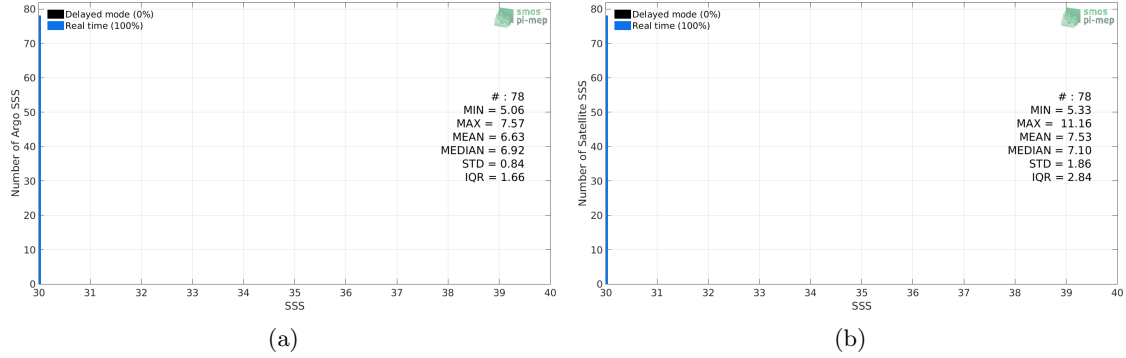
Figure 2: Histograms of SSS from Argo (a) and SMOS-L3-CATDS-CPDC-V317-MONTHLY-25KM (b) considering all match-up pairs per bins of 0.1 over the Baltic Sea Pi-MEP region and for the full satellite product period.
