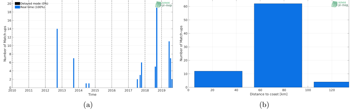
Figure 1: Number of match-ups between Argo and SMOS-L3-CATDS-CPDC-V317-MONTHLY-25KM SSS as a function of time (a) and as function of the distance to coast (b) over the Baltic Sea Pi-MEP region and for the full satellite product period.
