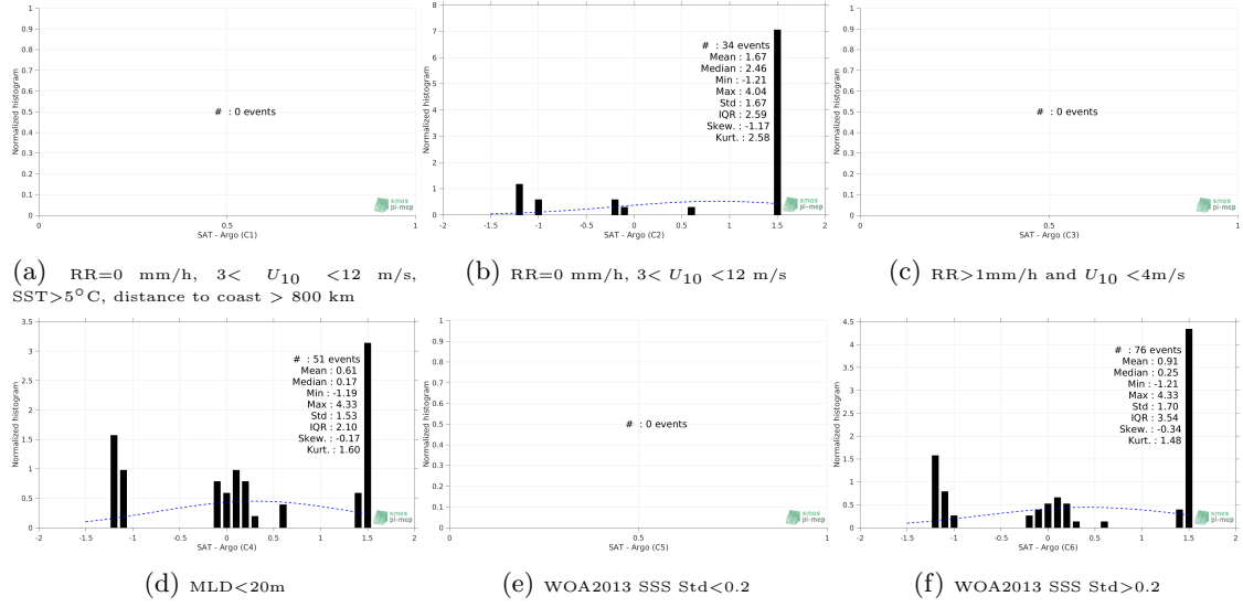
Figure 13: Normalized histogram of \Delta\text{SSS} (SMOS-L3-CATDS-CPDC-V317-MONTHLY-25KM - Argo) for 6 different subdatasets corresponding to: RR=0 mm/h, 3 < U_{10} < 12 m/s, SST > 5^\circ\text{C} , distance to coast > 800 km (a), RR=0 mm/h, 3 < U_{10} < 12 m/s (b), RR > 1\text{mm/h} and U_{10} < 4\text{m/s} (c), MLD < 20\text{m} (d), WOA2013 SSS Std < 0.2 (e), WOA2013 SSS Std > 0.2 (f).
