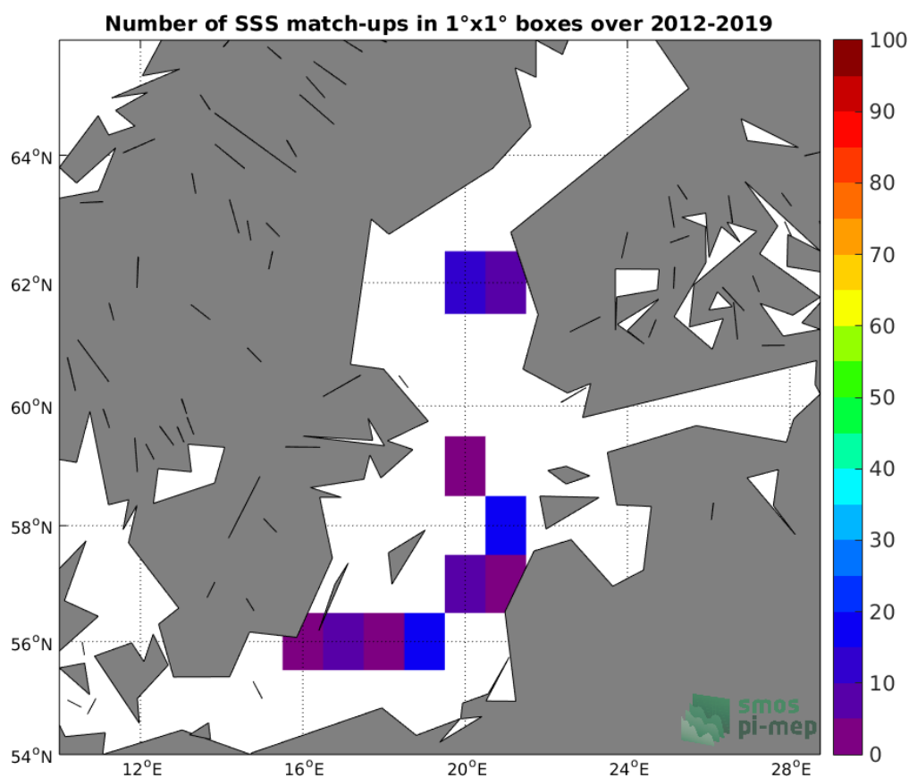
Figure 4: Number of SSS match-ups between Argo SSS and the SMOS-L3-CATDS-CPDC-V317-MONTHLY-25KM SSS product for the Baltic Sea Pi-MEP region over 1°x1° boxes and for the full satellite product period.
