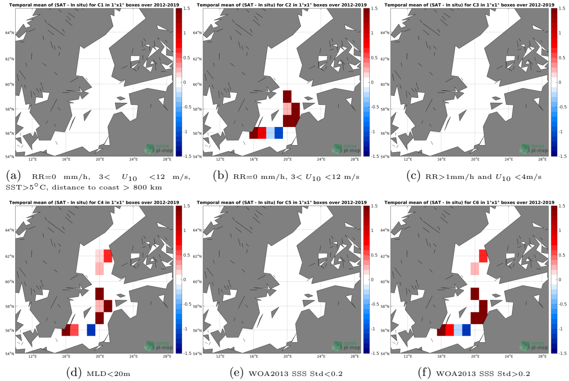
Figure 12: Temporal mean gridded over spatial boxes of size 1^\circ \times 1^\circ of \Delta SSS (SMOS-L3-CATDS-CPDC-V317-MONTHLY-25KM - Argo) for 6 different subdatasets corresponding to: RR=0 mm/h, 3 < U_{10} < 12 m/s, SST >5^\circ\text{C} , distance to coast > 800 km (a), RR=0 mm/h, 3 < U_{10} < 12 m/s (b), RR >1 mm/h and U_{10} < 4 m/s (c),MLD <20 m (d),WOA2013 SSS Std <0.2 (e),WOA2013 SSS Std >0.2 (f).
