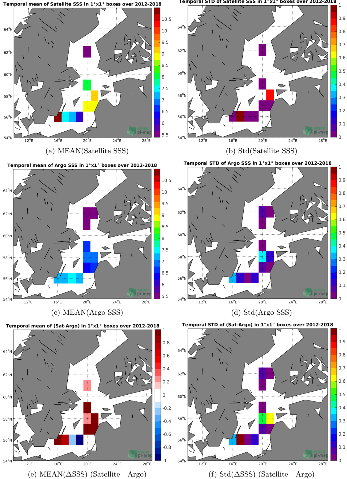
Figure 6: Temporal mean (left) and Std (right) of SSS from SMOS-L3-CATDS-CPDC-V317-MONTHLY-25KM (top), Argo (middle), and of \Delta SSS (Satellite - Argo). Only match-up pairs are used to generate these maps.
