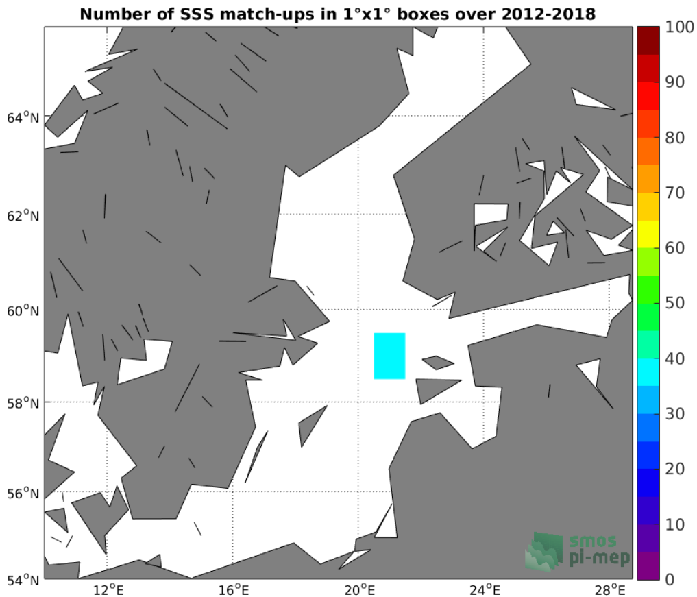
Figure 4: Number of SSS match-ups between TSG (LEGOS-DM) SSS and the SMOS SSS L3 v317 - 10 Days - 25 km (CATDS-CPDC) SSS product for the Baltic Sea Pi-MEP region over 1^\circ \times 1^\circ boxes and for the full satellite product period.
