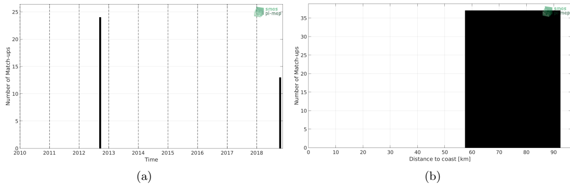
Figure 1: Number of match-ups between TSG (LEGOS-DM) and SMOS SSS L3 v317 - 10 Days - 25 km (CATDS-CPDC) SSS as a function of time (a) and as function of the distance to coast (b) over the Baltic Sea Pi-MEP region and for the full satellite product period.
