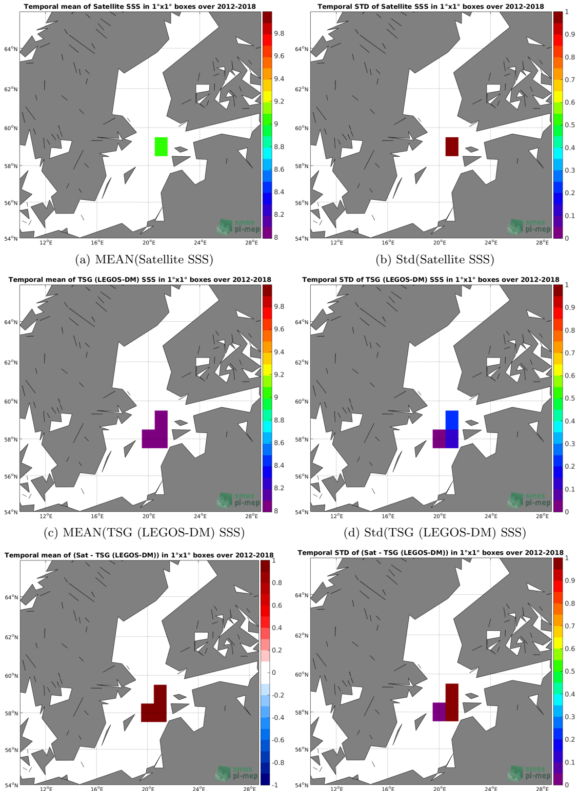
(e) MEAN( \Delta SSS) (Satellite - TSG (LEGOS-DM))
