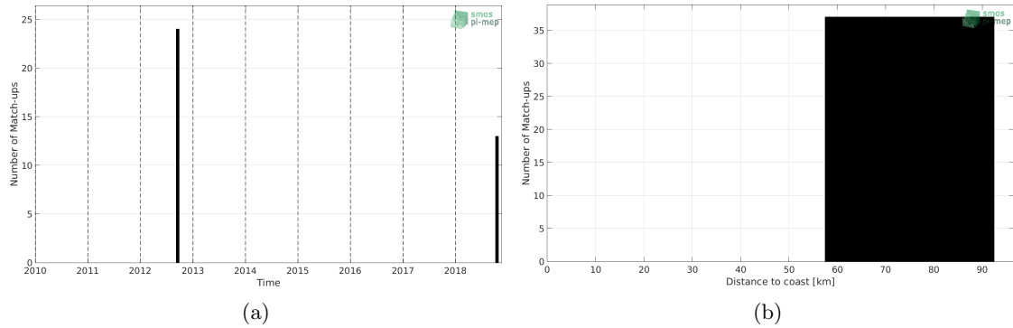
Figure 1: Number of match-ups between TSG (LEGOS-DM) and SMOS SSS L3 v317 - 10 Days - 25 km (CATDS-CPDC) SSS as a function of time (a) and as function of the distance to coast (b) over the Baltic Sea Pi-MEP region and for the full satellite product period.
