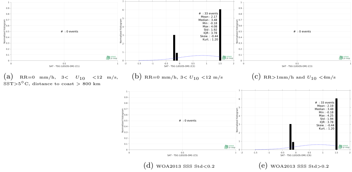
Figure 13: Normalized histogram of \Delta\text{SSS} (SMOS SSS L3 v317 - 10 Days - 25 km (CATDS-CPDC) - TSG (LEGOS-DM)) for 5 different subdatasets corresponding to: RR=0 mm/h, 3 < U_{10} < 12 m/s, SST > 5^{\circ}\text{C} , distance to coast > 800 km (a), RR=0 mm/h, 3 < U_{10} < 12 m/s (b), RR > 1\text{mm/h} and U_{10} < 4\text{m/s} (c), WOA2013 SSS Std < 0.2 (d), WOA2013 SSS Std > 0.2 (e).
