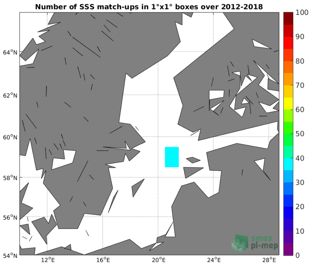
Figure 4: Number of SSS match-ups between TSG (LEGOS-DM) SSS and the SMOS SSS L3 v317 - 10 Days - 25 km (CATDS-CPDC) SSS product for the Baltic Sea Pi-MEP region over 1°x1° boxes and for the full satellite product period.
