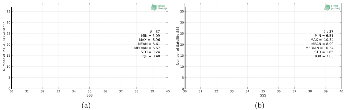
Figure 2: Histograms of SSS from TSG-LEGOS-DM (a) and SMOS L3 v317 - 10 Days - 25 km (CATDS-CPDC) (b) considering all match-up pairs per bins of 0.1 over the Baltic Sea Pi-MEP region and for the full satellite product period.
