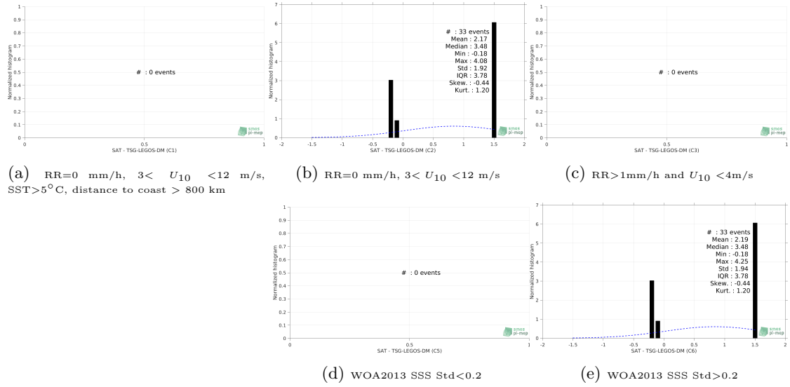
Figure 13: Normalized histogram of \Delta SSS (SMOS L3 v317 - 10 Days - 25 km (CATDS-CPDC) - TSG-LEGOS-DM) for 5 different subdatasets corresponding to: RR=0 mm/h, 3 < U_{10} < 12 m/s, SST>5°C, distance to coast > 800 km (a), RR=0 mm/h, 3 < U_{10} < 12 m/s (b), RR>1mm/h and U_{10} < 4 m/s (c), WOA2013 SSS Std<0.2 (d), WOA2013 SSS Std>0.2 (e).
