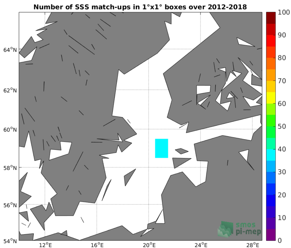
Figure 4: Number of SSS match-ups between TSG-LEGOS-DM SSS and the SMOS L3 v317 - 10 Days - 25 km (CATDS-CPDC) SSS product for the Baltic Sea Pi-MEP region over 1°x1° boxes and for the full satellite product period.
