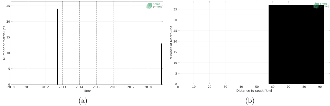
Figure 1: Number of match-ups between TSG-LEGOS-DM and SMOS L3 v317 - 10 Days - 25 km (CATDS-CPDC) SSS as a function of time (a) and as function of the distance to coast (b) over the Baltic Sea Pi-MEP region and for the full satellite product period.
