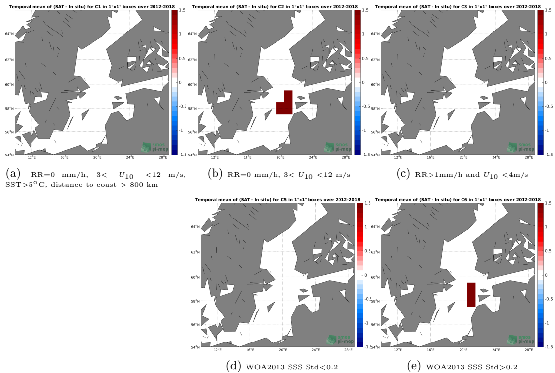
Figure 12: Temporal mean gridded over spatial boxes of size 1^{\circ}\times 1^{\circ} of \Delta\text{SSS} (SMOS L3 v317 - 10 Days - 25 km (CATDS-CPDC) - TSG-LEGOS-DM) for 5 different subdatasets corresponding to:RR=0 mm/h, 3 < U_{10} < 12 m/s, SST >5^{\circ}\text{C} , distance to coast > 800 km (a), RR=0 mm/h, 3 < U_{10} < 12 m/s (b), RR >1 mm/h and U_{10} < 4 m/s (c), WOA2013 SSS Std <0.2 (d), WOA2013 SSS Std >0.2 (e).
