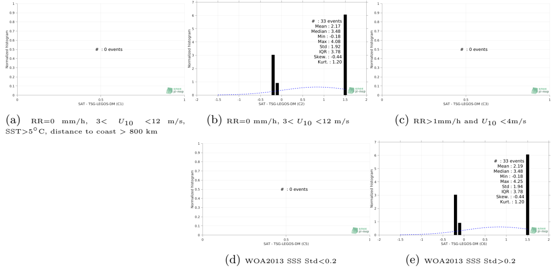
Figure 13: Normalized histogram of \Delta SSS (SMOS-L3-CATDS-CPDC-V317-10DAYS-25KM - TSG-LEGOS-DM) for 5 different subdatasets corresponding to: RR=0 mm/h, 3 < U_{10} < 12 m/s, SST>5°C, distance to coast > 800 km (a), RR=0 mm/h, 3 < U_{10} < 12 m/s (b), RR>1mm/h and U_{10} < 4 m/s (c), WOA2013 SSS Std<0.2 (d), WOA2013 SSS Std>0.2 (e).
