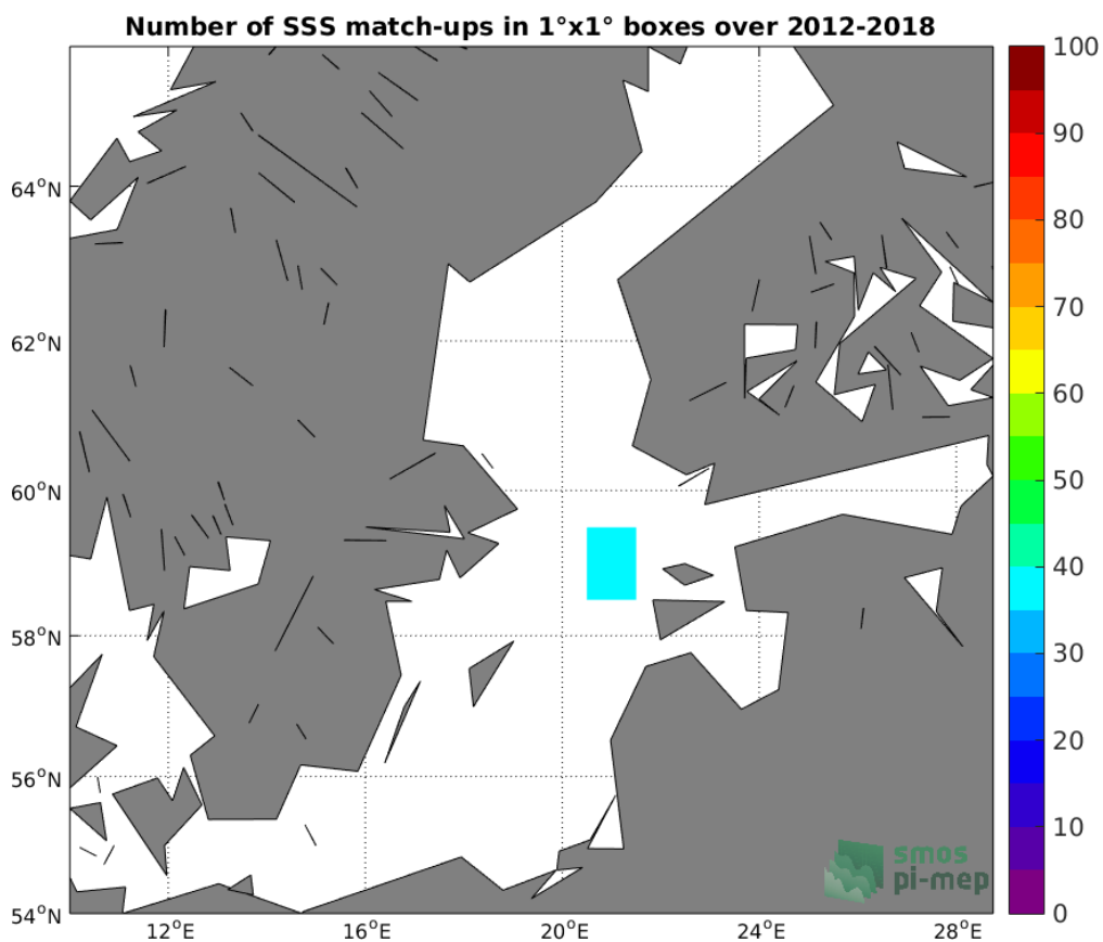
Figure 4: Number of SSS match-ups between TSG-LEGOS-DM SSS and the SMOS-L3-CATDS-CPDC-V317-10DAYS-25KM SSS product for the Baltic Sea Pi-MEP region over 1°x1° boxes and for the full satellite product period.
