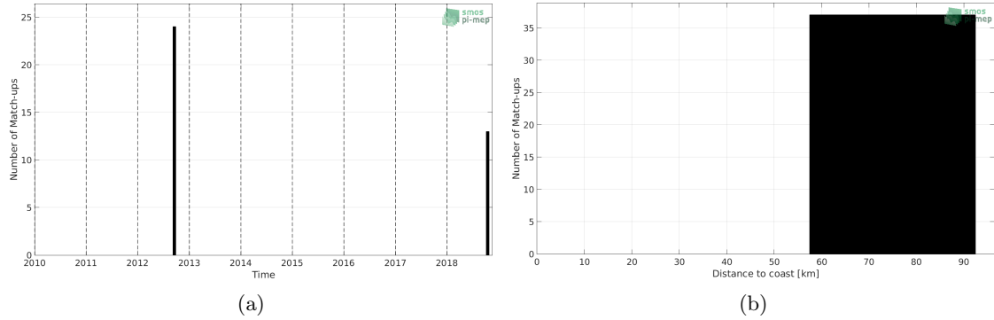
Figure 1: Number of match-ups between TSG-LEGOS-DM and SMOS-L3-CATDS-CPDC-V317-10DAYS-25KM SSS as a function of time (a) and as function of the distance to coast (b) over the Baltic Sea Pi-MEP region and for the full satellite product period.
