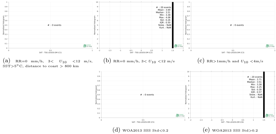
Figure 13: Normalized histogram of \Delta\text{SSS} (SMOS-L3-CATDS-CPDC-V317-10DAYS-25KM - TSG-LEGOS-DM) for 5 different subdatasets corresponding to: RR=0 mm/h, 3 < U_{10} < 12 m/s, SST > 5^\circ\text{C} , distance to coast > 800 km (a), RR=0 mm/h, 3 < U_{10} < 12 m/s (b), RR > 1\text{mm/h} and U_{10} < 4\text{m/s} (c), WOA2013 SSS Std < 0.2 (d), WOA2013 SSS Std > 0.2 (e).
