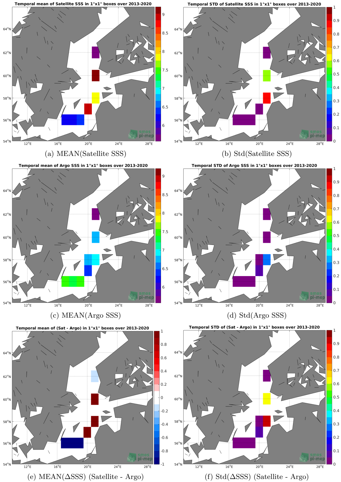
Figure 6: Temporal mean (left) and Std (right) of SSS from SMOS SSS L3 v317 - 10 Days - 25 km (CATDS-CPDC) (top), Argo (middle), and \Delta SSS (Satellite - Argo). Only match-up pairs are used to generate these maps.
