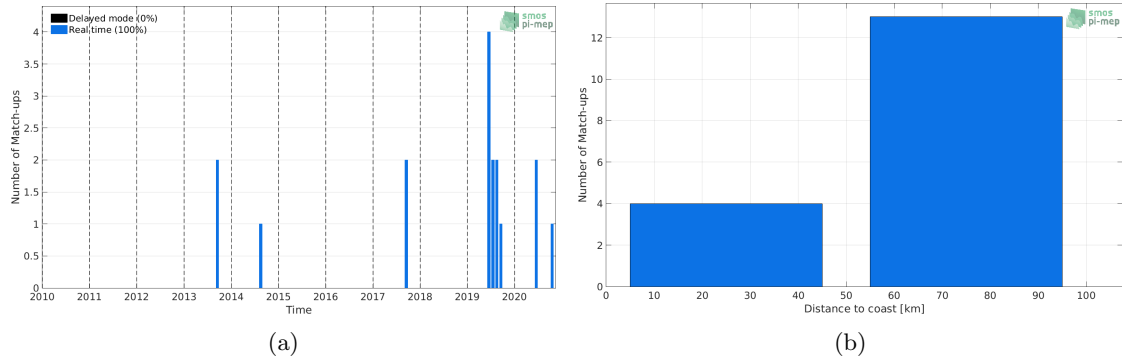
Figure 1: Number of match-ups between Argo and SMOS SSS L3 v317 - 10 Days - 25 km (CATDS-CPDC) SSS as a function of time (a) and as function of the distance to coast (b) over the Baltic Sea Pi-MEP region and for the full satellite product period.
