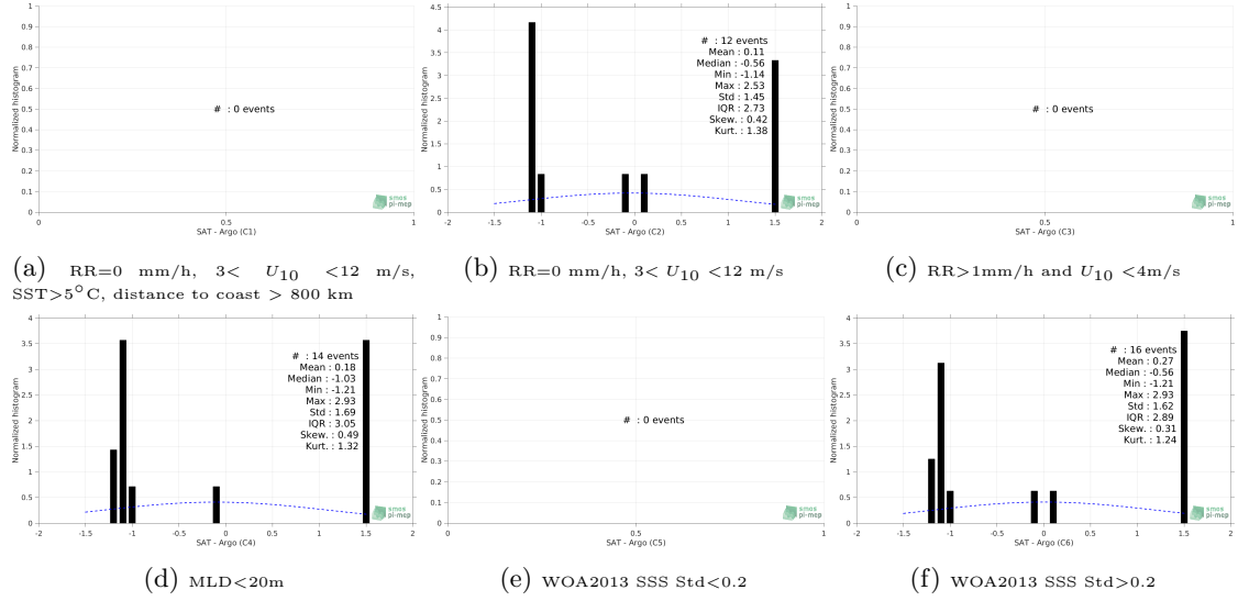
Figure 13: Normalized histogram of \Delta SSS (SMOS SSS L3 v317 - 10 Days - 25 km (CATDS-CPDC) - Argo) for 6 different subdatasets corresponding to: RR=0 mm/h, 3 < U_{10} < 12 m/s, SST >5^{\circ} C, distance to coast > 800 km (a), RR=0 mm/h, 3 < U_{10} < 12 m/s (b), RR >1 mm/h and U_{10} < 4 m/s (c), MLD <20 m (d), WOA2013 SSS Std <0.2 (e), WOA2013 SSS Std >0.2 (f).
