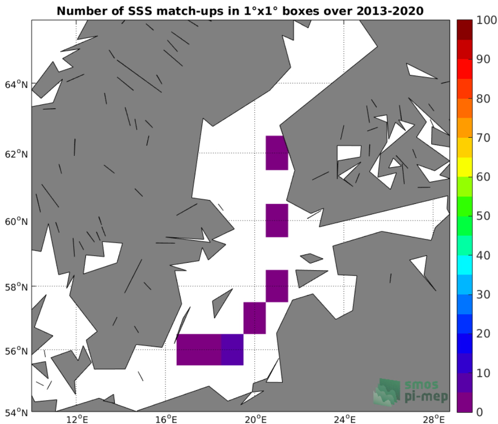
Figure 4: Number of SSS match-ups between Argo SSS and the SMOS SSS L3 v317 - 10 Days - 25 km (CATDS-CPDC) SSS product for the Baltic Sea Pi-MEP region over 1°x1° boxes and for the full satellite product period.
