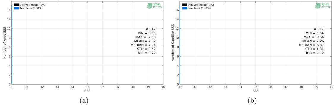
Figure 2: Histograms of SSS from Argo (a) and SMOS SSS L3 v317 - 10 Days - 25 km (CATDS-CPDC) (b) considering all match-up pairs per bins of 0.1 over the Baltic Sea Pi-MEP region and for the full satellite product period.
