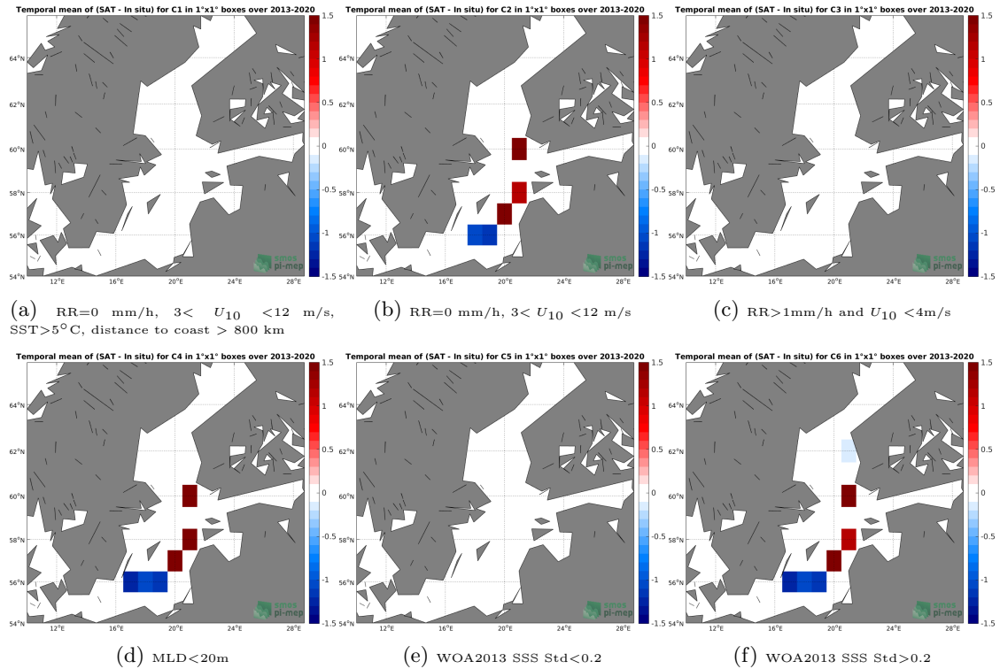
Figure 12: Temporal mean gridded over spatial boxes of size 1^{\circ}\times 1^{\circ} of \Delta\text{SSS} (SMOS SSS L3 v317 - 10 Days - 25 km (CATDS-CPDC) - Argo) for 6 different subdatasets corresponding to:RR=0 mm/h, 3 < U_{10} < 12 m/s, SST > 5^{\circ}\text{C} , distance to coast > 800 km (a), RR=0 mm/h, 3 < U_{10} < 12 m/s (b), RR > 1\text{mm/h} and U_{10} < 4\text{m/s} (c),MLD < 20\text{m} (d),WOA2013 SSS Std < 0.2 (e),WOA2013 SSS Std > 0.2 (f).
