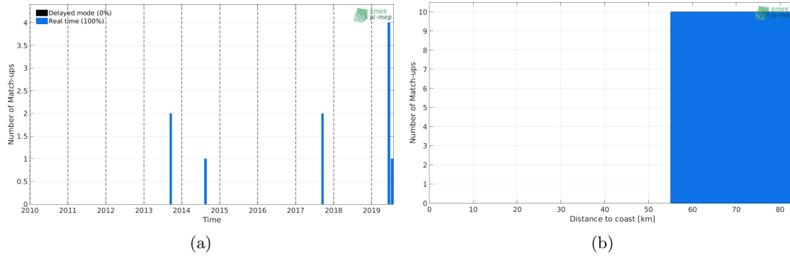
Figure 1: Number of match-ups between Argo and SMOS-L3-CATDS-CPDC-V317-10DAYS-25KM SSS as a function of time (a) and as function of the distance to coast (b) over the Baltic Sea Pi-MEP region and for the full satellite product period.
