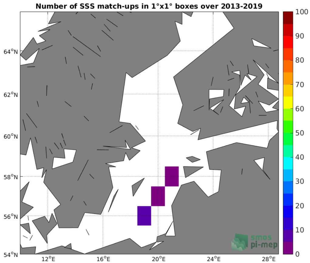
Figure 4: Number of SSS match-ups between Argo SSS and the SMOS-L3-CATDS-CPDC-V317-10DAYS-25KM SSS product for the Baltic Sea Pi-MEP region over 1°x1° boxes and for the full satellite product period.
