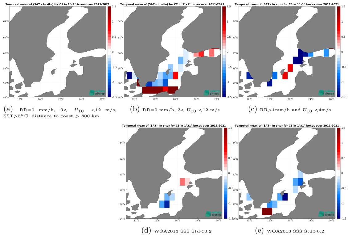
Figure 14: Temporal mean gridded over spatial boxes of size 1^\circ \times 1^\circ of \Delta\text{SSS} (SMOS SSS L3 v2 - 9-Days (BEC) - TSG (LEGOS-DM)) for 5 different subdatasets corresponding to:RR=0 mm/h, 3 < U_{10} < 12 m/s, SST > 5°C, distance to coast > 800 km (a), RR=0 mm/h, 3 < U_{10} < 12 m/s (b), RR > 1mm/h and U_{10} < 4 m/s (c), WOA2013 SSS Std < 0.2 (d), WOA2013 SSS Std > 0.2 (e).
