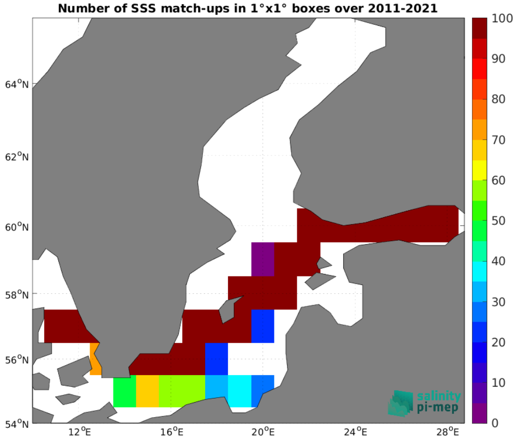
Figure 4: Number of SSS match-ups between TSG (LEGOS-DM) SSS and the SMOS SSS L3 v2 - 9-Days (BEC) SSS product for the Baltic Sea Pi-MEP region over 1^\circ \times 1^\circ boxes and for the full satellite product period.
