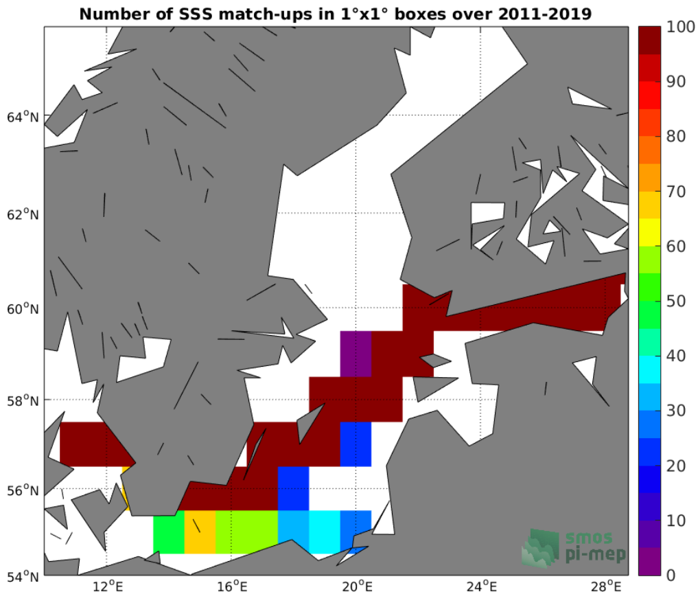
Figure 4: Number of SSS match-ups between TSG (LEGOS-DM) SSS and the SMOS SSS L3 v2 - 9-Days (BEC) SSS product for the Baltic Sea Pi-MEP region over 1°×1° boxes and for the full satellite product period.
