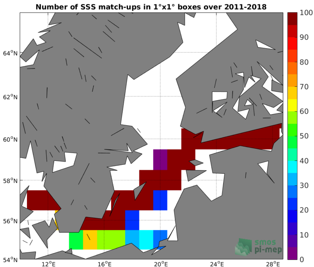
Figure 4: Number of SSS match-ups between TSG (LEGOS-DM) SSS and the SMOS L3 v2 - 9-Days (BEC) SSS product for the Baltic Sea Pi-MEP region over 1°x1° boxes and for the full satellite product period.
