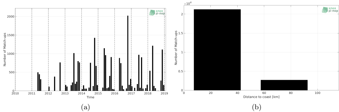
Figure 1: Number of match-ups between TSG (LEGOS-DM) and SMOS L3 v2 - 9-Days (BEC) SSS as a function of time (a) and as function of the distance to coast (b) over the Baltic Sea Pi-MEP region and for the full satellite product period.
