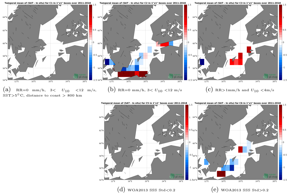
Figure 12: Temporal mean gridded over spatial boxes of size 1^{\circ}\times 1^{\circ} of \Delta\text{SSS} (SMOS L3 v2 - 9-Days (BEC) - TSG (LEGOS-DM)) for 5 different subdatasets corresponding to:RR=0 mm/h, 3 < U_{10} < 12 m/s, SST >5^{\circ}\text{C} , distance to coast > 800 km (a), RR=0 mm/h, 3 < U_{10} < 12 m/s (b), RR >1 mm/h and U_{10} < 4 m/s (c), WOA2013 SSS Std <0.2 (d), WOA2013 SSS Std >0.2 (e).
