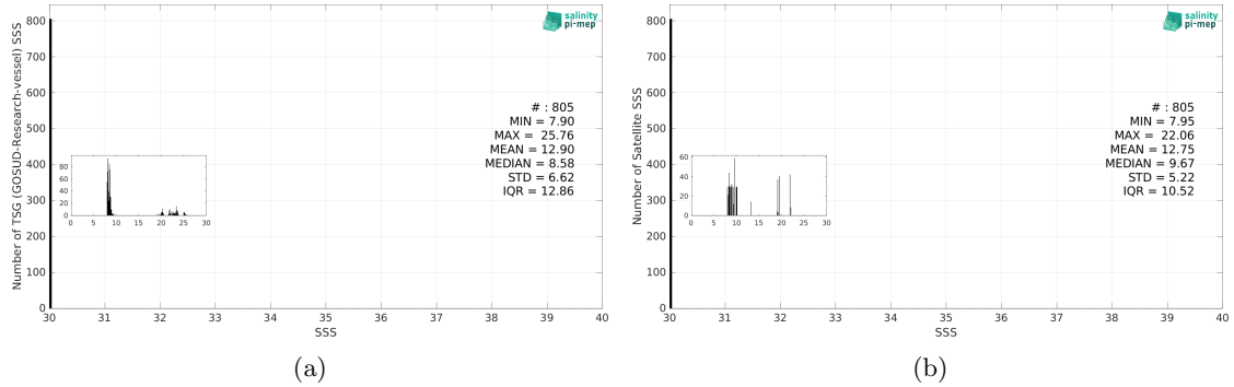
Figure 3: Histograms of SSS from TSG (GOSUD-Research-vessel) (a) and SMOS SSS L3 v2 - 9-Days (BEC) (b) considering all match-up pairs per bins of 0.1 over the Baltic Sea Pi-MEP region and for the full satellite product period.
