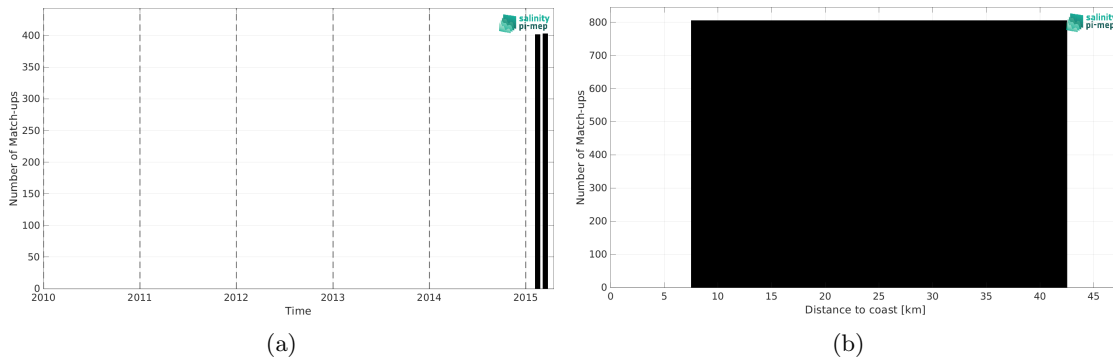
Figure 2: Number of match-ups between TSG (GOSUD-Research-vessel) and SMOS SSS L3 v2 - 9-Days (BEC) SSS as a function of time (a) and as function of the distance to coast (b) over the Baltic Sea Pi-MEP region and for the full satellite product period.
