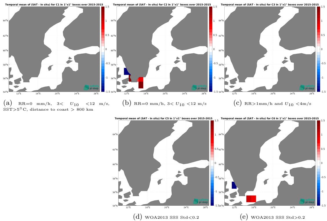
Figure 14: Temporal mean gridded over spatial boxes of size 1^\circ \times 1^\circ of \Delta SSS (SMOS SSS L3 v2 - 9-Days (BEC) - TSG (GOSUD-Research-vessel)) for 5 different subdatasets corresponding to:RR=0 mm/h, 3 < U_{10} < 12 m/s, SST >5^\circ C, distance to coast > 800 km (a), RR=0 mm/h, 3 < U_{10} < 12 m/s (b), RR >1 mm/h and U_{10} < 4 m/s (c), WOA2013 SSS Std <0.2 (d), WOA2013 SSS Std >0.2 (e).
