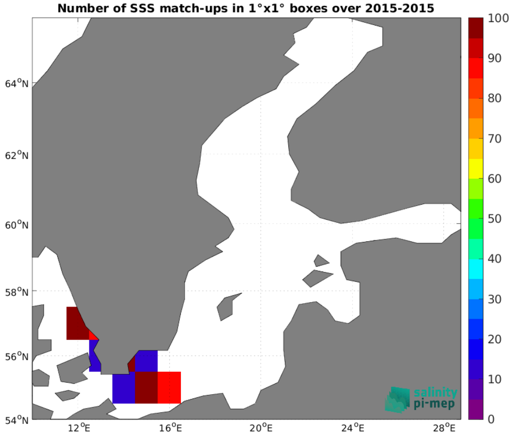
Figure 5: Number of SSS match-ups between TSG (GOSUD-Research-vessel) SSS and the SMOS SSS L3 v2 - 9-Days (BEC) SSS product for the Baltic Sea Pi-MEP region over 1^\circ \times 1^\circ boxes and for the full satellite product period.
