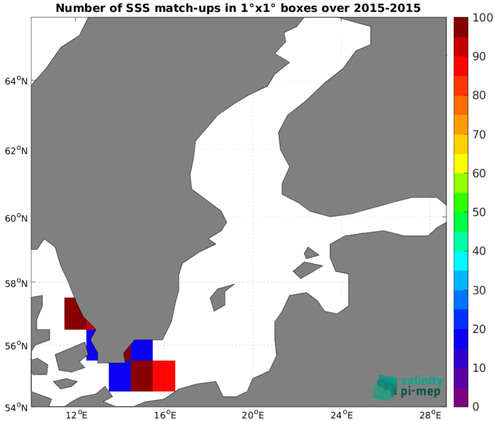
Figure 4: Number of SSS match-ups between TSG (GOSUD-Research-vessel) SSS and the SMOS SSS L3 v2 - 9-Days (BEC) SSS product for the Baltic Sea Pi-MEP region over 1^\circ \times 1^\circ boxes and for the full satellite product period.
