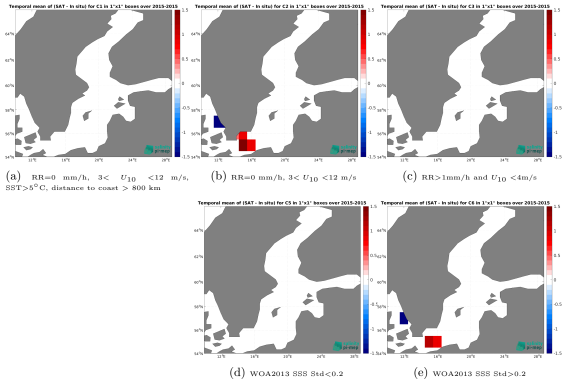
Figure 12: Temporal mean gridded over spatial boxes of size 1^\circ \times 1^\circ of \Delta SSS (SMOS SSS L3 v2 - 9-Days (BEC) - TSG (GOSUD-Research-vessel)) for 5 different subdatasets corresponding to: RR=0 mm/h, 3 < U_{10} < 12 m/s, SST > 5^\circ\text{C} , distance to coast > 800 km (a), RR=0 mm/h, 3 < U_{10} < 12 m/s (b), RR > 1 mm/h and U_{10} < 4 m/s (c), WOA2013 SSS Std < 0.2 (d), WOA2013 SSS Std > 0.2 (e).
